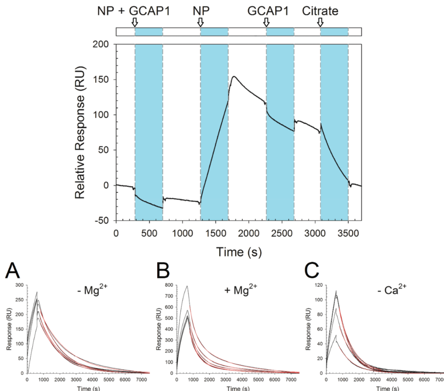
Fig. 6 SPR experiments. Top: Sensorgram of sequential injections over immobilized WT GCAP1 of, respectively: 0.3 mg ml -1 CaF 2 NP incubated with 5 μM WT GCAP1; 0.3 mg ml -1 NP; 5 μM WT GCAP1; 10 mM K-citrate. Bottom: Sensorgram of the injections of 0.1, 0.2, 0.3, 0.4, and 0.5 mg ml -1 NP over immobilized D100E GCAP1. NP were dissolved in (A) 5 mM Tris/HCl pH 7.5, 150 mM KCl, (B) 5 mM Tris/HCl pH 7.5, 150 mM KCl, 1 mM Mg 2+ , (C) decalcified 5 mM Tris/HCl pH 7.5, 150 mM KCl.
