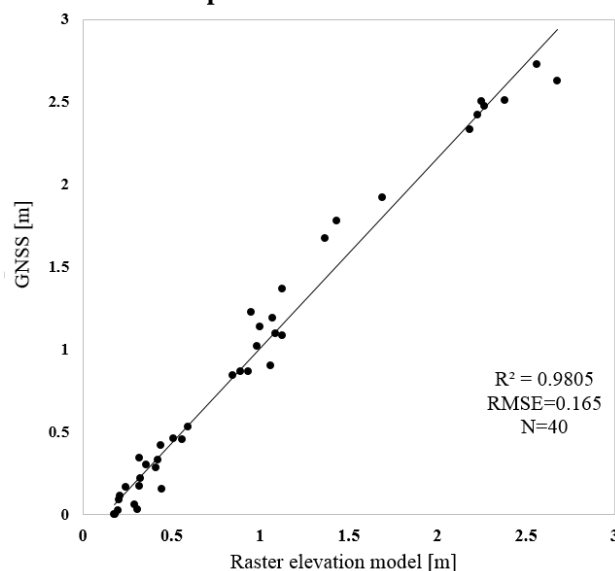
Figure 9. Top : 2D Displacement [m] coloured map obtained by ABM process on the DSM with related movements vectors calculated automatically (using a 10 pixel grid step). Bottom : Scatterplot between displacements obtained from the automatic comparison of UAS and GNSS measurements on 40 points
