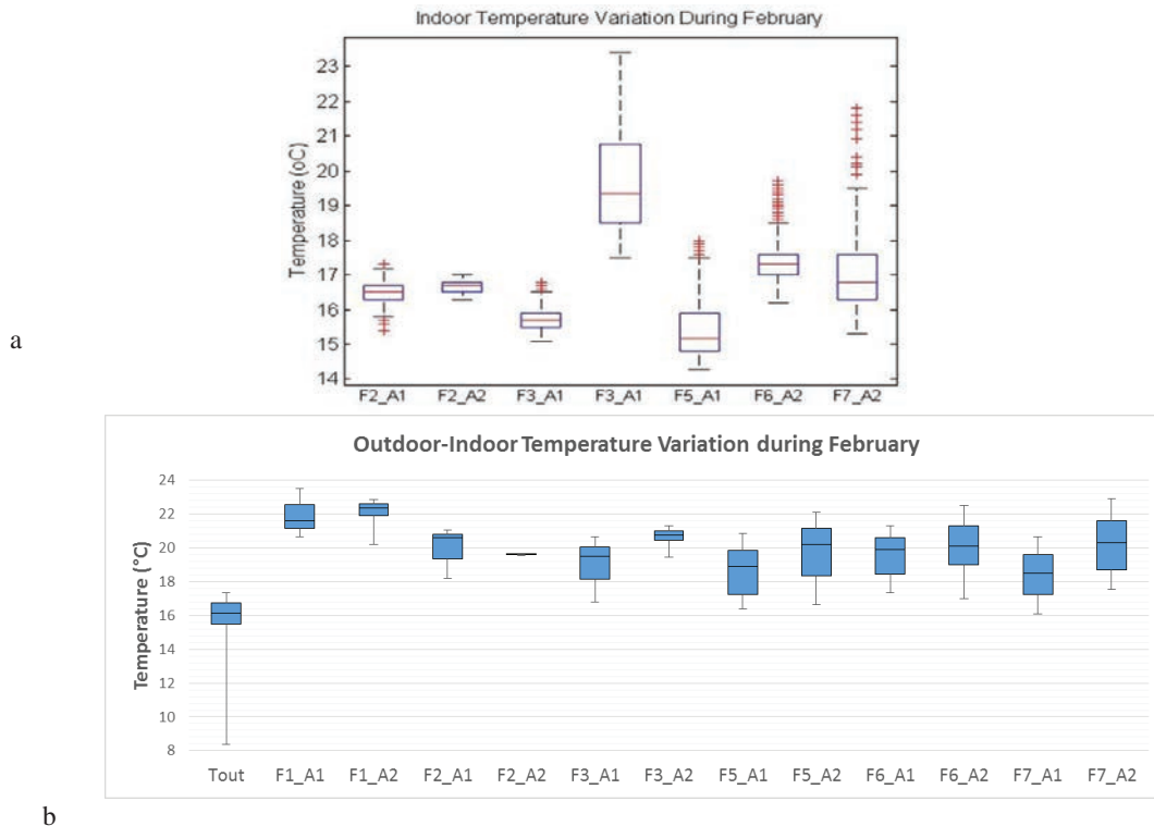
Fig.7. Box plot of the indoor and outdoor temperature for February for the apartments pre retrofit (A) and post retrofit (B).
