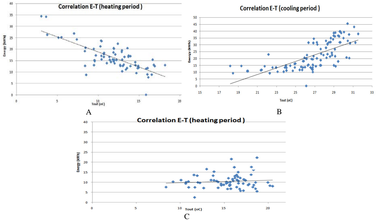
Fig. 6. Energy signature for the Greek building for the heating (A) and cooling season (B) before the retrofit and for the heating season after the retrofit (C)
