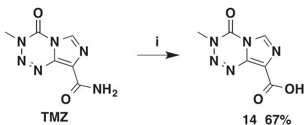
Scheme 6. Reagents and conditions: (i) \text{Con. H}_2\text{SO}_4 , \text{NaNO}_2 , 0\text{ }^\circ\text{C} – 15\text{ }^\circ\text{C} .
