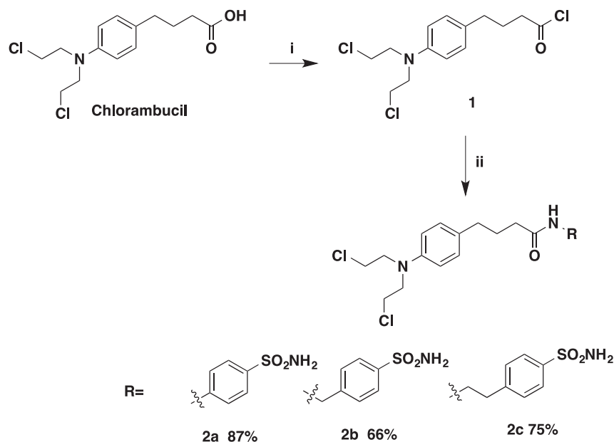
Scheme 1. Reagents and conditions: (i) (COCl)_2 , DMF, DCM, 0^\circ C –rt; (ii) DIPEA, THF, 0^\circ C –rt.
