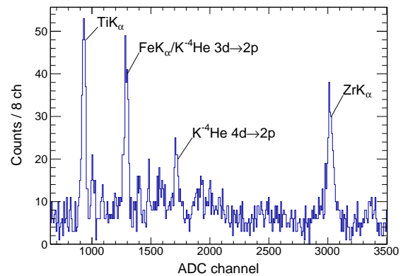
Fig. 2. Typical ADC spectrum of 1 SDD readout channel with the helium-4 target in E62.
