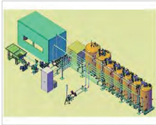
Figure 2. Multi stage fermentation pilot plant
