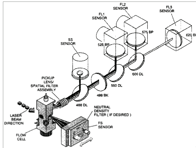
Figure 3: Schematic diagram flow cytometry (Coulter, 1996 [4])
