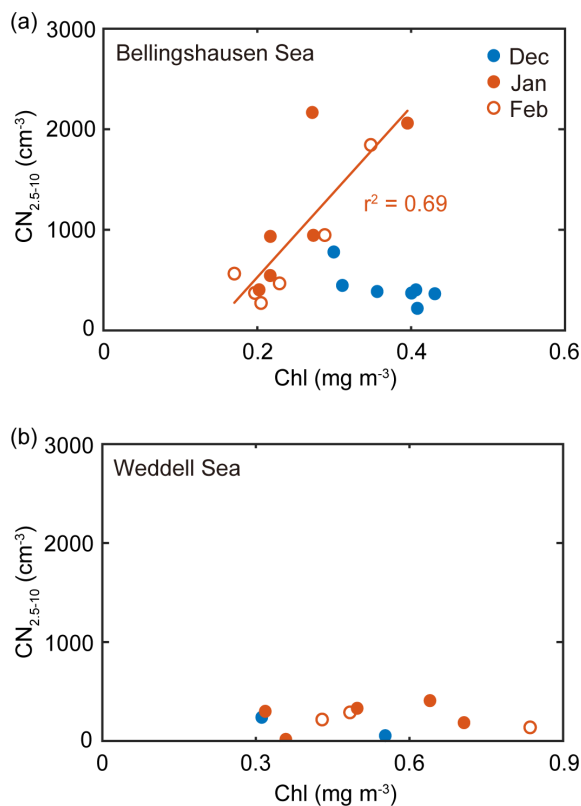
Figure 5. (a) Relationship between the monthly mean chlorophyll concentration for the Bellingshausen Sea (55–65° S, 60–80° W) and the monthly mean number concentration of nanoparticles that originated from the Bellingshausen Sea in 2009–2016. (b) Relationship between the monthly mean chlorophyll concentration for the Weddell Sea (55–65° S, 40–60° W) and the monthly mean number concentration of nanoparticles that originated from the Weddell Sea in 2009–2016. The filled blue, filled red and open red symbols indicate the data obtained in December, January and February, respectively. The solid lines represent the best fit.
