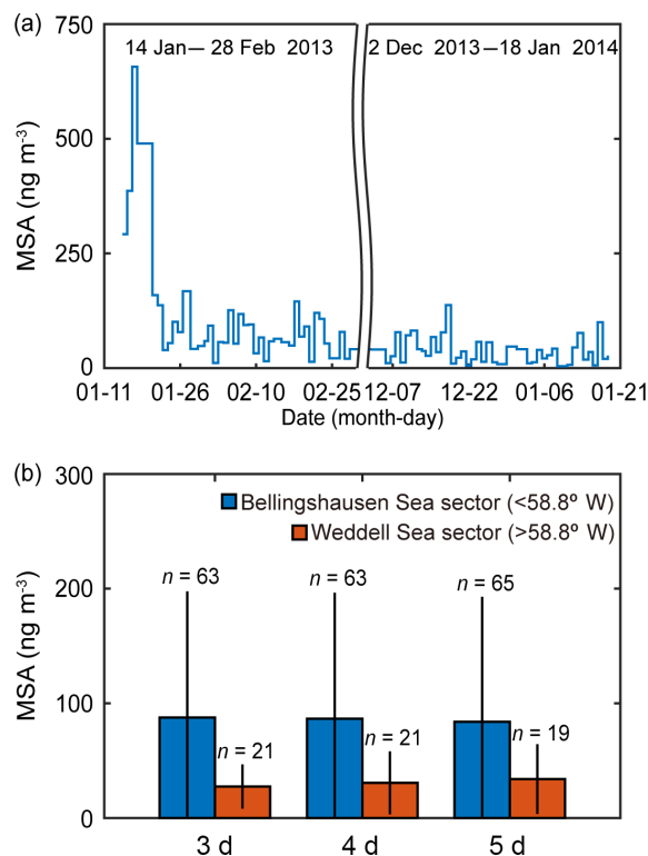
Figure 4. (a) Daily concentration of MSA collected at the sampling site during the summer periods in 2013 and 2014 (explicitly, from 14 January to 28 February in 2013 and from 2 December 2013 to 18 January 2014). (b) The mean MSA concentration that potentially originated from the Bellingshausen Sea sector (< 58.8° W) and the Weddell Sea sector (> 58.8° W) estimated by applying 3, 4 and 5 d air mass back trajectories during the austral summer periods in 2013 and 2014. The error bars indicate 1 standard deviation ( 1\sigma ) from the mean values.
