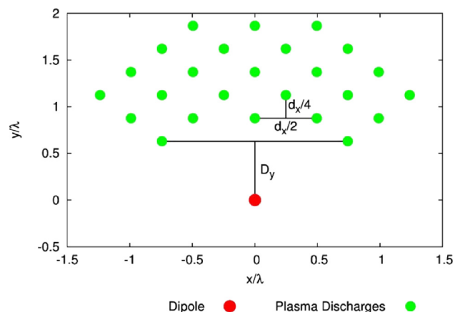
Fig. 2. Top view of the transmit-array antenna layout.
