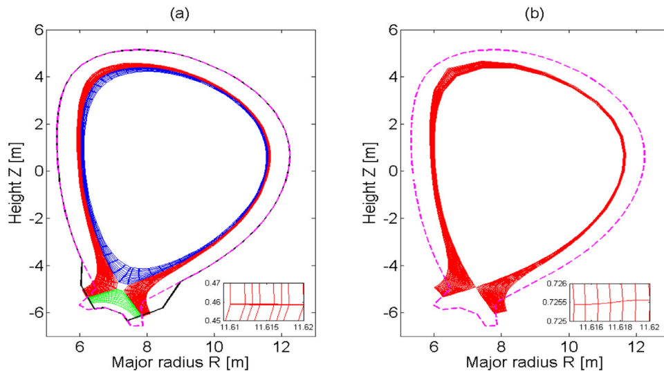
Fig. 1. (a) Mesh used in EDGE2D-EIRENE for the simulation of the SOL plasma. The main SOL is depicted in red, the Private region in green and the external core corona in blue. The black line denotes the vessel geometry used in the simulations. (b) Mesh used in the TECXY simulations. The magenta dashed lines indicate the actual geometry of the vessel. In both the figures the zoom of the grids at the OMP is shown in the lower right corners. (For interpretation of the references to colour in this figure legend, the reader is referred to the web version of this article.)
