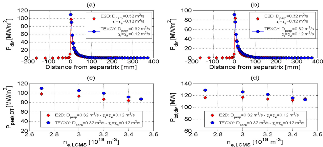
Fig. 4. Profiles of power onto the outer divertor as a function of the distance from the separatrix obtained with EDGE2D-EIRENE and TECXY (red diamonds and blue circles respectively) by imposing (a) n_{e,LCMS} = 2.7 \times 10^{19} \text{ m}^{-3} and (b) n_{e,LCMS} = 3.4 \times 10^{19} \text{ m}^{-3} . (c) Power peaks on the outer target and (d) total power reaching the inner and outer divertor plates as a function of the OMP electron density. The input parameters are P_{SOL} = 150 \text{ MW} , diffusion coefficients D^{\perp} = 0.32 \text{ m}^2/\text{s} and \chi = 0.12 \text{ m}^2/\text{s} . (For interpretation of the references to colour in this figure legend, the reader is referred to the web version of this article.)
