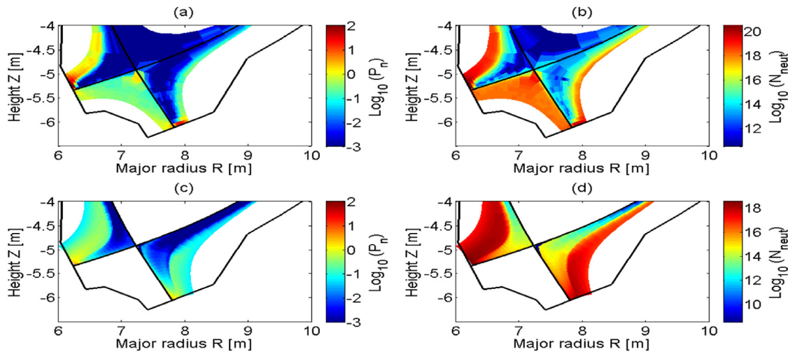
Fig. 3. 2D contour maps of the neutral pressure (a), (c) and of the neutral density (b), (d) in the divertor area plotted in log scale. The figures on the top refer to the EDGE2D-EIRENE calculations while the ones on the bottom to TECXY. The input parameters are n_{e,LCMS} = 2.7 \times 10^{19} \text{ m}^{-3} , P_{SOL} = 150 \text{ MW} , D^{\perp} = 0.32 \text{ m}^2/\text{s} and \chi = 0.12 \text{ m}^2/\text{s} .
