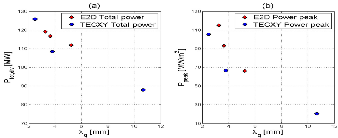
Fig. 5. (a) Total power onto the divertor plates and (b) power peaks as a function of the power e-folding length at the OMP obtained with EDGE2D-EIRENE (red diamonds) and TECXY (blue circles) by imposing n_{e,LCMS} = 3 \times 10^{19} \text{ m}^{-3} and P_{SOL} = 150 \text{ MW} . (For interpretation of the references to colour in this figure legend, the reader is referred to the web version of this article.)
