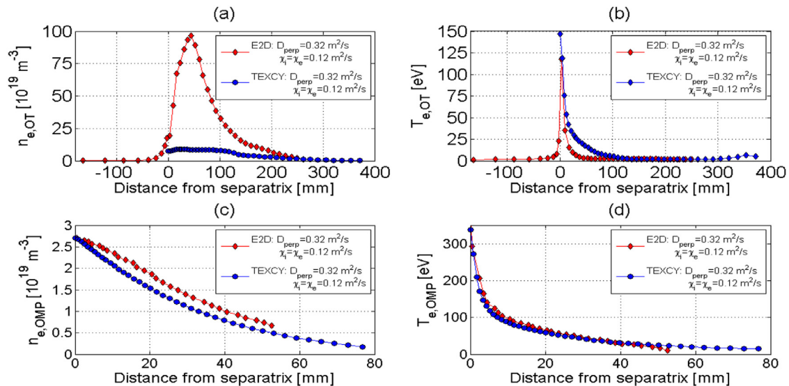
Fig. 2. Profiles of (a) the electron density and of (b) the electron temperature at the outer target as a function of the distance from the separatrix obtained with EDGE2D-EIRENE and TECXY (red diamonds and blue circles, respectively). The input parameters in the simulation are n_{e,LCMS} = 2.7 \times 10^{19} \text{ m}^{-3} , P_{SOL} = 150 \text{ MW} and diffusion coefficients D_{\perp} = 0.32 \text{ m}^2/\text{s} and \chi = 0.12 \text{ m}^2/\text{s} . The profiles of (c) n_e and (d) T_e at the OMP are also shown.
