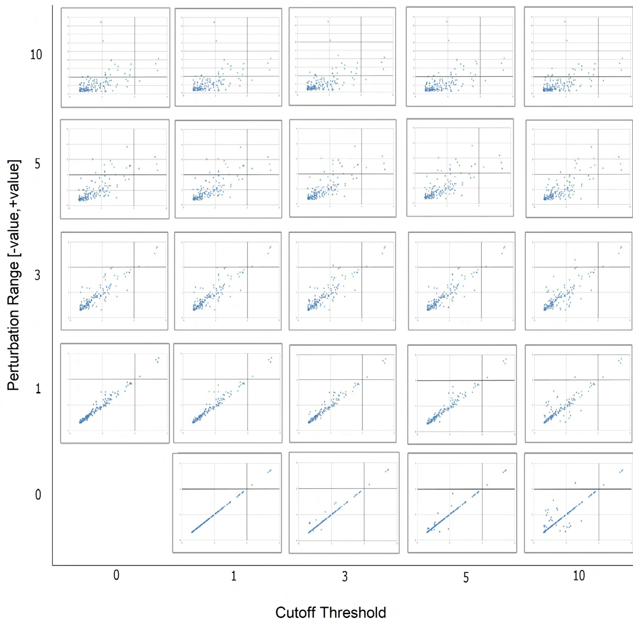
Fig. 1. Cut-off and perturbation evaluation graphs. Each cut-off and perturbation parameter combination is represented by a graph at the relevant cell in the figure. The resulting -\log(\text{p-value}) are plotted against the results of the corresponding tests with no perturbation or cut-off applied (no added noise). The bold vertical and horizontal lines indicate in each graph the a-priori statistical significance threshold
