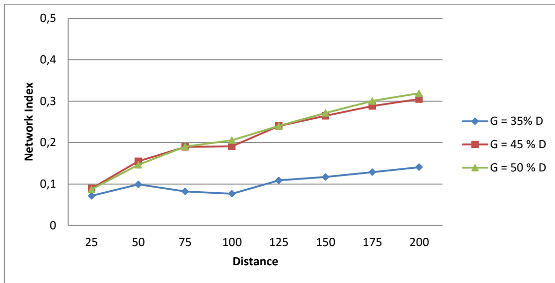
Fig. 3. Network Index by varying the distance d of connection for different percentage of energy generation
