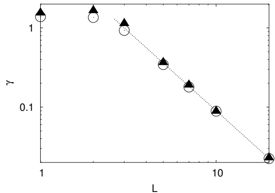
FIG. 2: Asymptotic exponential decay rates of fidelity for the sawtooth map ( K_0 = (\sqrt{5} + 1)/2 , \epsilon = 10^{-3} ) as a function of L . The rates are extracted by fitting the tails of the fidelity decay in the Fig. 1 (triangles) and from the discretized Perron-Frobenius operator (circles). The line denotes the \propto 1/L^2 behavior of the decay rates, as predicted by the Fokker-Planck equation.
