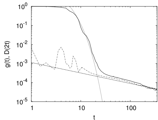
FIG. 4: Decay of fidelity for the kicked rotator with K_0 = 2.5 , L = 1 , and \epsilon = 10^{-3} (full curve). The support of the initial (characteristic) density is (q, p) \in [0, 0.2] \times [0, 0.2] . The dotted curve gives the exponential decay determined by the Lyapunov coefficient (about 0.534), while the dashed line shows the \propto t^{-0.55} behavior. The decay of correlator D for the same initial density and for twice the time t is also shown (dot-dashed curve).
