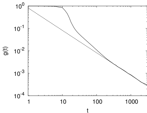
FIG. 3: Decay of fidelity for the stadium billiard with radius R = 1 and length of the straight segments d_0 = 2 (the perturbed stadium has d = d_0 + \epsilon , with \epsilon = 2 \times 10^{-3} ). The initial phase space density was chosen to be a direct product of a characteristic function on a circle in configuration space, the center of which was at (0.5, 0.25) as measured from the center of the billiard and its radius was 0.1, while for momenta the \delta(|\mathbf{p}| - 1) distribution was used. The dashed line represents the expected \propto 1/t decay of fidelity.
