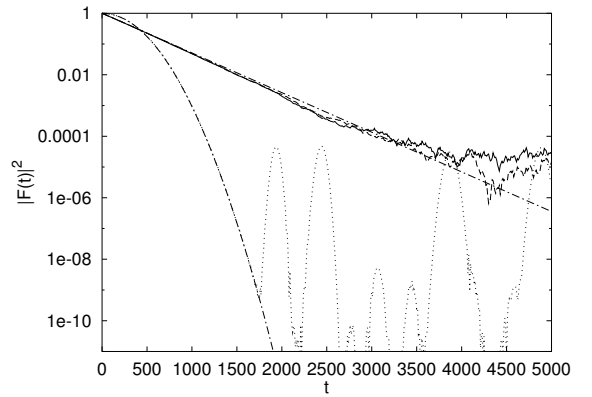
FIG. 5: Fidelity for two coupled kicked tops, \delta = 8 \cdot 10^{-4} and J = 200 . The upper curves are for \epsilon = 20 (mixing regime), solid curve for a coherent initial state and dashed curve for a random initial state, and the lower - dotted curve is for \epsilon = 1 (non-mixing regime) with a coherent initial state. The exponential and gaussian chain curves give, respectively, the expected theoretical decays (9) and (12).
