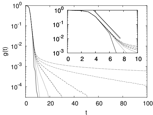
FIG. 1: Decay of the fidelity g(t) for the sawtooth map with the parameters K_0 = (\sqrt{5} + 1)/2 and \epsilon = 10^{-3} for different values of L = 1, 3, 5, 7, 10, 20, \infty from the fastest to the slowest decaying curve, respectively. The initial phase space density is chosen as the characteristic function on the support given by the (q, p) \in [0, 2\pi] \times [-\pi/100, \pi/100] . Note that between the Lyapunov decay and the exponential asymptotic decay there is a \propto 1/\sqrt{t} decay, as expected from diffusive behavior. Inset: magnification of the same plot for short times, with the corresponding Lyapunov decay indicated as a thick dashed line.
