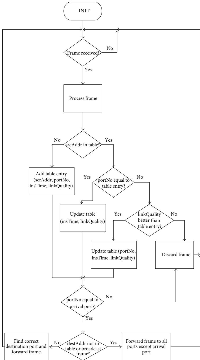
FIGURE 4: Switch flow chart.
