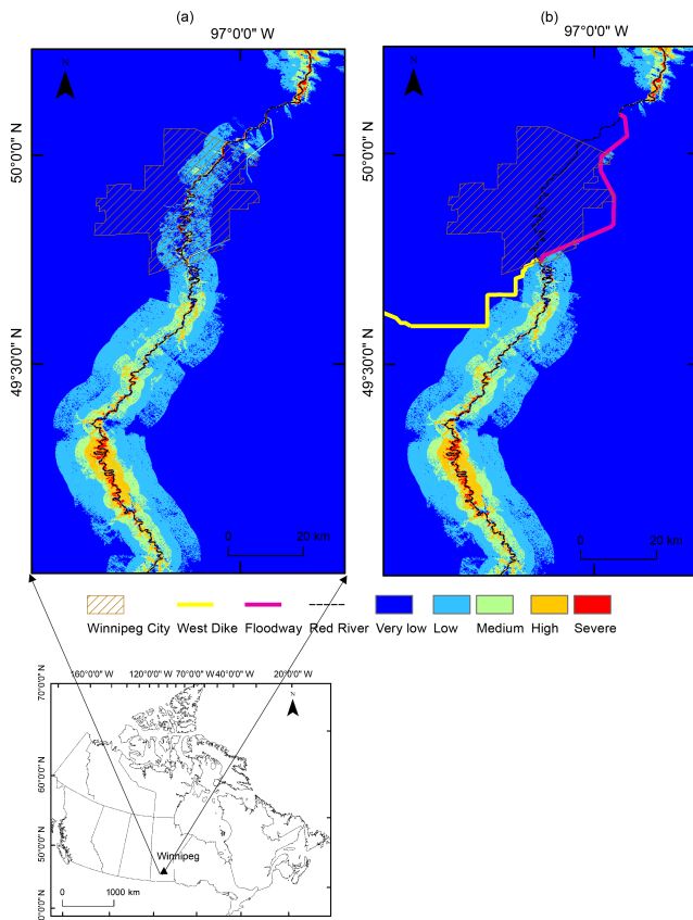
Figure 6. Hazard map for the Red River in Manitoba: (a) without considering flood protection structures in delineating hazard zones and (b) considering flood protection.
