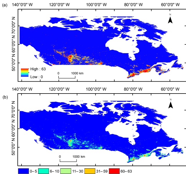
Figure 2. Nightlights over Canada shown as (a) continuous spectrum and (b) classified as shown in Table 3 into very low luminosity (0–5), low luminosity (6–10), medium luminosity (11–30), high luminosity (31–59), and very high luminosity (60–63).
