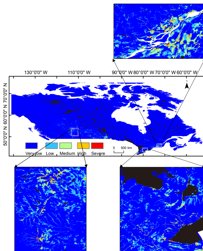
Figure 8. Flood risk map for Canada. Certain portions of the map are enlarged for better visual interpretation of the various levels of flood risk. The risk map is a product of hazard and exposure (flood protection measures are not included). Severe risk only occurs in areas of severe hazard and exposure, causing severe flood risk areas to be concentrated in urban centres.
