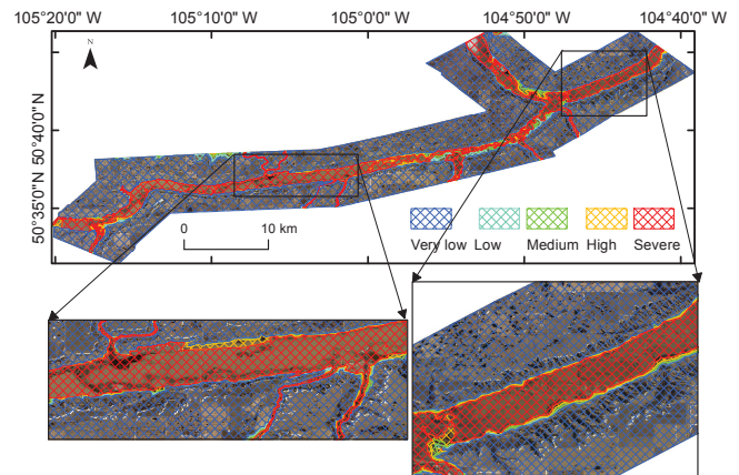
Figure 5. Comparison of hazard map with aerial image of a single flood event on the Qu'Appelle River, Saskatchewan (background). Date of image: 6 May 2013.
