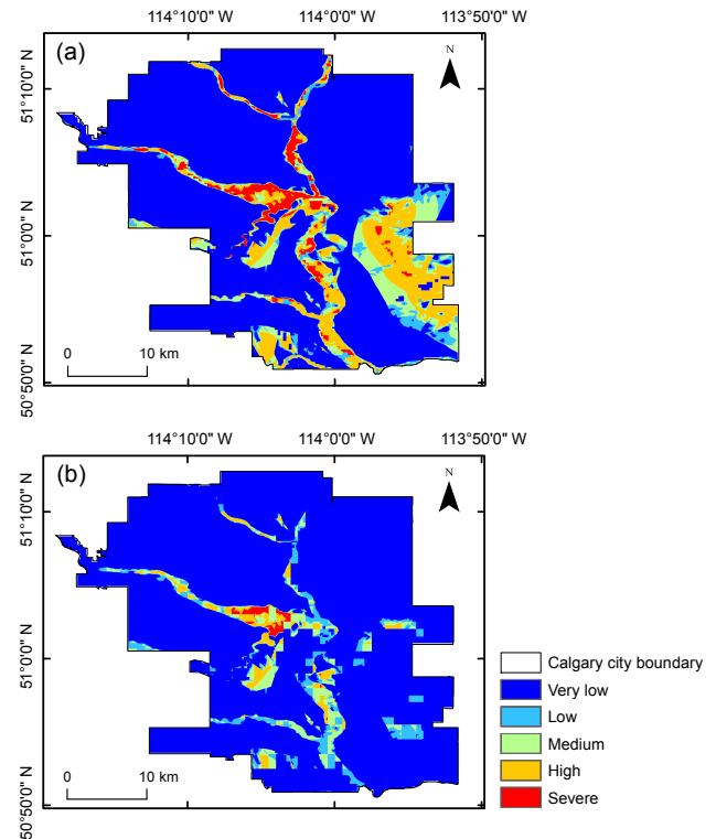
Figure 10. Flood risk map of Calgary: (a) without population information, and (b) with population. Areas around the centre of the city with high rises and dense population remain in the severe risk category, whereas northern and southern parts, which are mainly commercial, change to reduced levels of social risk.
