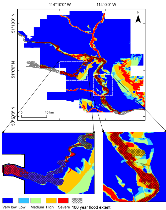
Figure 4. Comparison of hazard map obtained from the present study and a 100-year-flooding extent map prepared by the city of Calgary (hatched portions). Portions of the reach along the Bow and Elbow rivers are enlarged to show the level of agreement between both maps.
