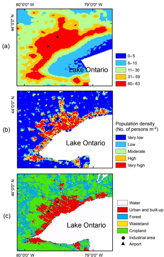
Figure 9. Comparison of population distribution and nightlights over Greater Toronto Area: (a) classified nightlights for the area with locations of the airport and a major industrial area, (b) population density over the area, and (c) land-use map of the area indicating urban extent.
