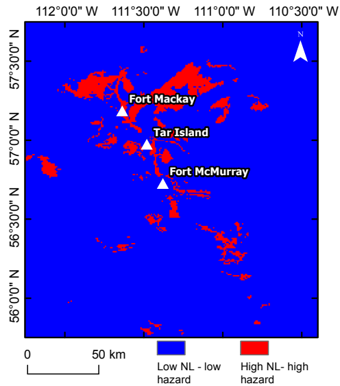
Figure 1. Locations indicating increase in nightlight (NL) activity over high-hazard areas between the years 1992 and 2013 ( DN_{2013} - DN_{1992} ).
