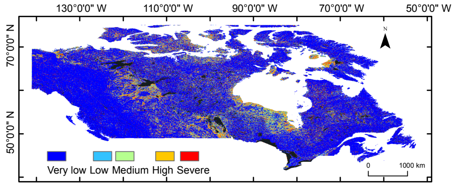
Figure 3. Flood hazard map for Canada obtained using the 20 m DEM. Large areas are classified under high- and severe-level flood hazard, but most areas have negligible human presence and investments.
