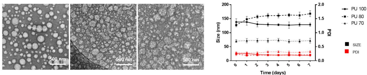
Figure 2 a) TEM analysis of PU100, PU80, and PU70 nanoparticles (scale bars represent 500 nm); b) PNPs stability curve over 7 days of incubation in saline, evaluated as a daily measurement of size (black curves) and PDI (red curves).
