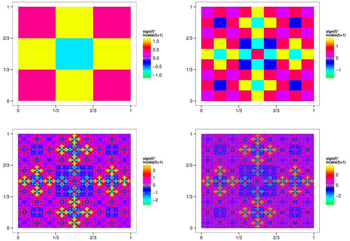
Figure 2: Density f of \mathcal{W}_{\tau_2}^n(I) , with \tau_2 according to Example 2.2 and n \in \{1, 2, 4, 6\}
