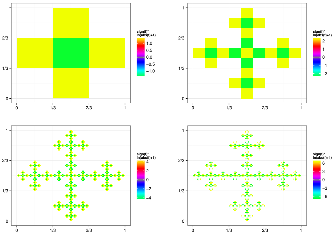
Figure 1: Density f of \mathcal{W}_{\tau_1}^n(I) , with \tau_1 according to Example 2.1 and n \in \{1, 2, 4, 6\}
