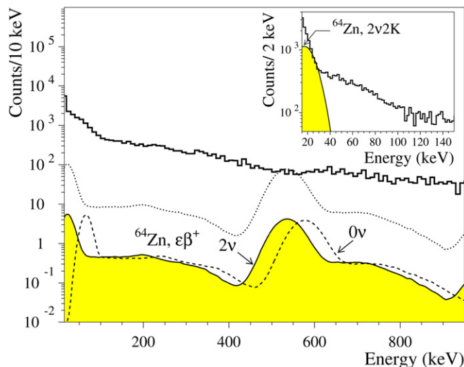
Fig. 2. The measured energy spectrum of the \text{ZnWO}_4 scintillation crystal (mass of 117 g, 1902 h of measurements)—corrected for the energy dependence of detection efficiency—together with the distributions for \epsilon\beta^+ processes in ^{64}\text{Zn} excluded at 90% C.L. Energy spectrum of 2\nu\epsilon\beta^+ decay with T_{1/2} = 1.1 \times 10^{19} yr (central value of positive indication in Ref. [11]) is also shown by dotted line. In the Inset: Low energy part of the spectrum together with the 2\nu 2K peak of ^{64}\text{Zn} with T_{1/2} = 6.2 \times 10^{18} yr excluded at 90% C.L.
