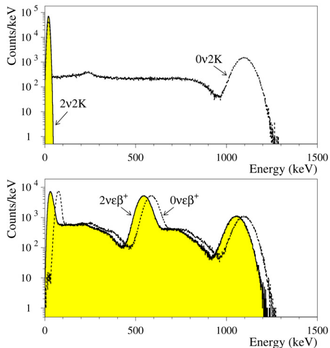
Fig. 3. Simulated response functions of the \text{ZnWO}_4 scintillator for different \epsilon\beta^+ and 2e decays in ^{64}\text{Zn} . One million of decays was simulated for each mode.
