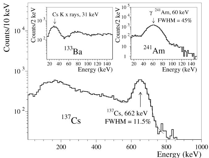
Fig. 1. Energy spectra measured by \text{ZnWO}_4 detector with ^{137}\text{Cs} (main part), and ^{133}\text{Ba} and ^{241}\text{Am} (insets) \gamma sources.
