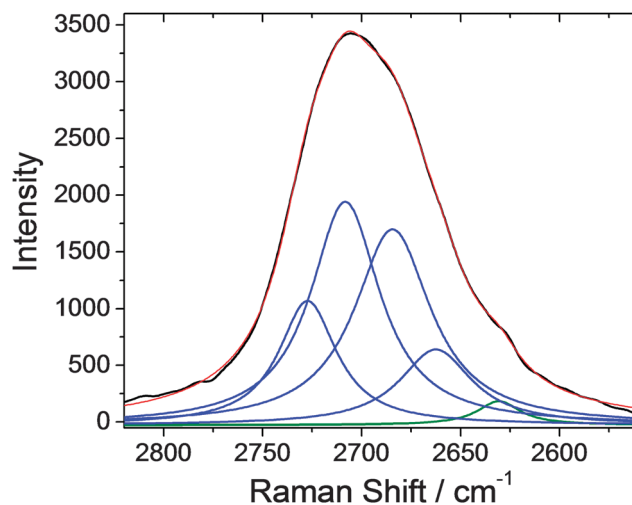
Fig. 6 Raman spectra of mesoporous silica films in the range 2820–2560 cm -1 containing exfoliated graphene and gold nanoparticles, thermally treated at 350 °C. The black curve shows the acquired Raman spectrum while the red line describes the fitting obtained by combining the Lorentzian curves (blue curves). The green line centred at 2625 cm -1 is the fitted band of the silicon signal.
