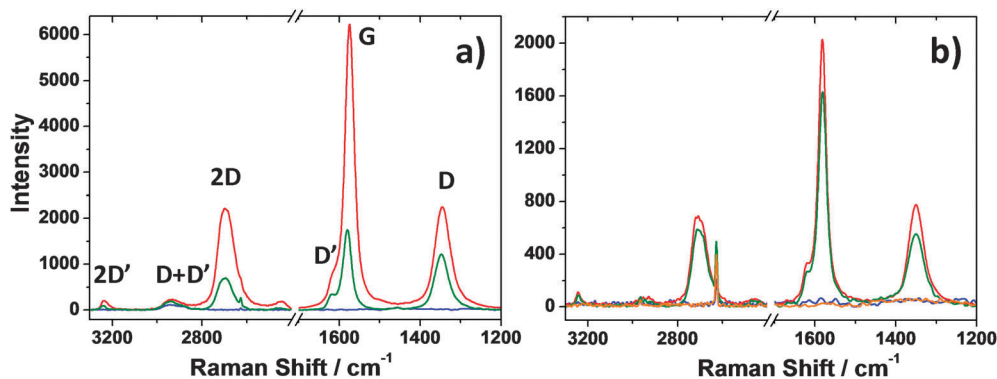
Fig. 5 Raman spectra in the 3300–1200 cm -1 range of mesoporous silica films and films containing either graphene or gold or both, thermally treated at 100 (a) and 350 °C (b). Blue line: mesoporous silica films; red line: mesoporous silica films containing exfoliated graphene; orange line: mesoporous silica films containing gold nanoparticles; green line: mesoporous silica films containing both exfoliated graphene and gold nanoparticles.
