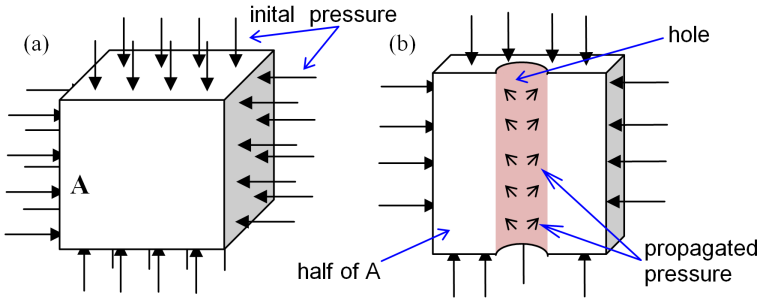
Fig. 10. Fluid pressure propagation in case of mesh drilling.
