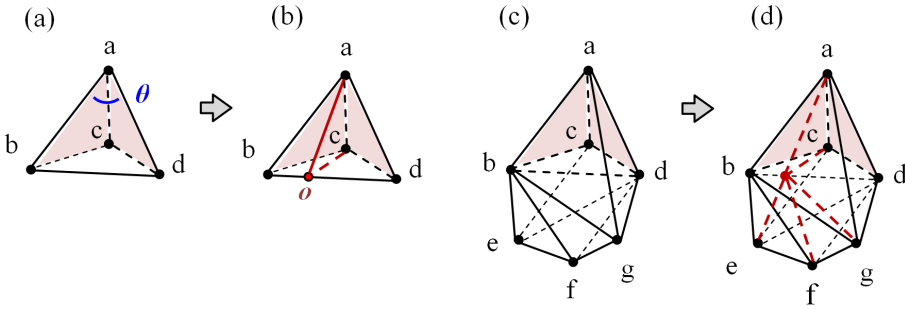
Fig. 12. Splitting schema for the tetrahedron with 2 potential interface triangles.
