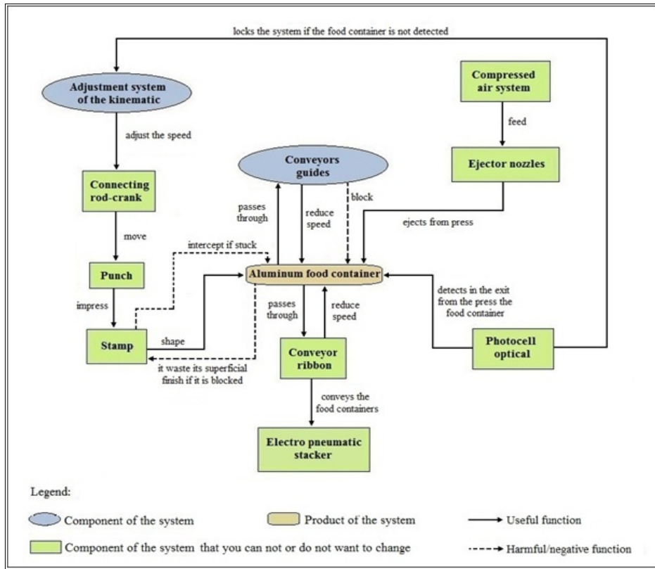
Figure 4. System functional model
