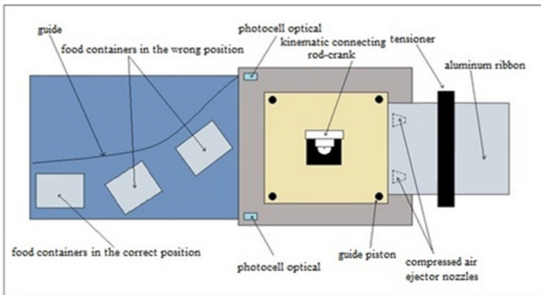
Figure 11. Proposed solution with the vibrating ribbon
