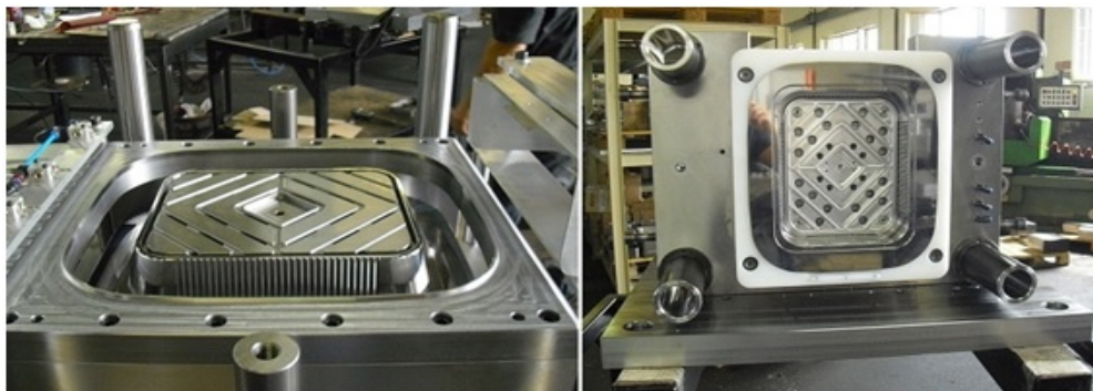
Figure. 3. Matrix and punch of a stamp for aluminum food containers
