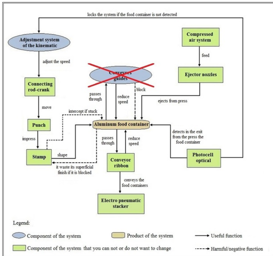
Figure 5. Examination of the system functional model without the conveyors guides
