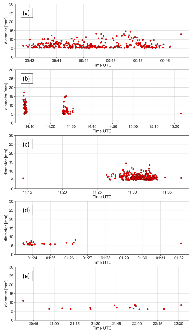
Figure 3. Time series of hailstone impacts; the y axis shows the estimated diameter (mm). Note the different timescales on the x axis. (a) 8 July 2021 at Trafohaus, Bironico. (b) 24 July 2021 at Mösl, Marbach. (c) 26 July 2021 at Bergstation Marbachegg. (d) 2 August 2019 at Onecars, Lugano. (e) 6 August 2021 at Scuola Elementare Cadro.
