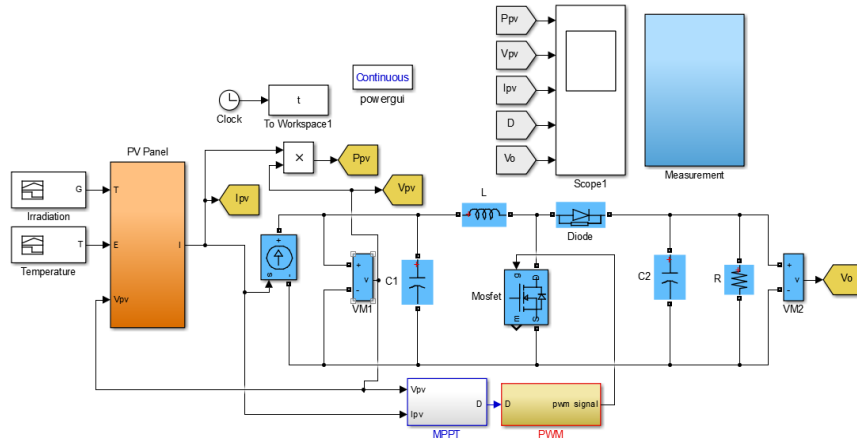
Fig. 7. PV System Model
