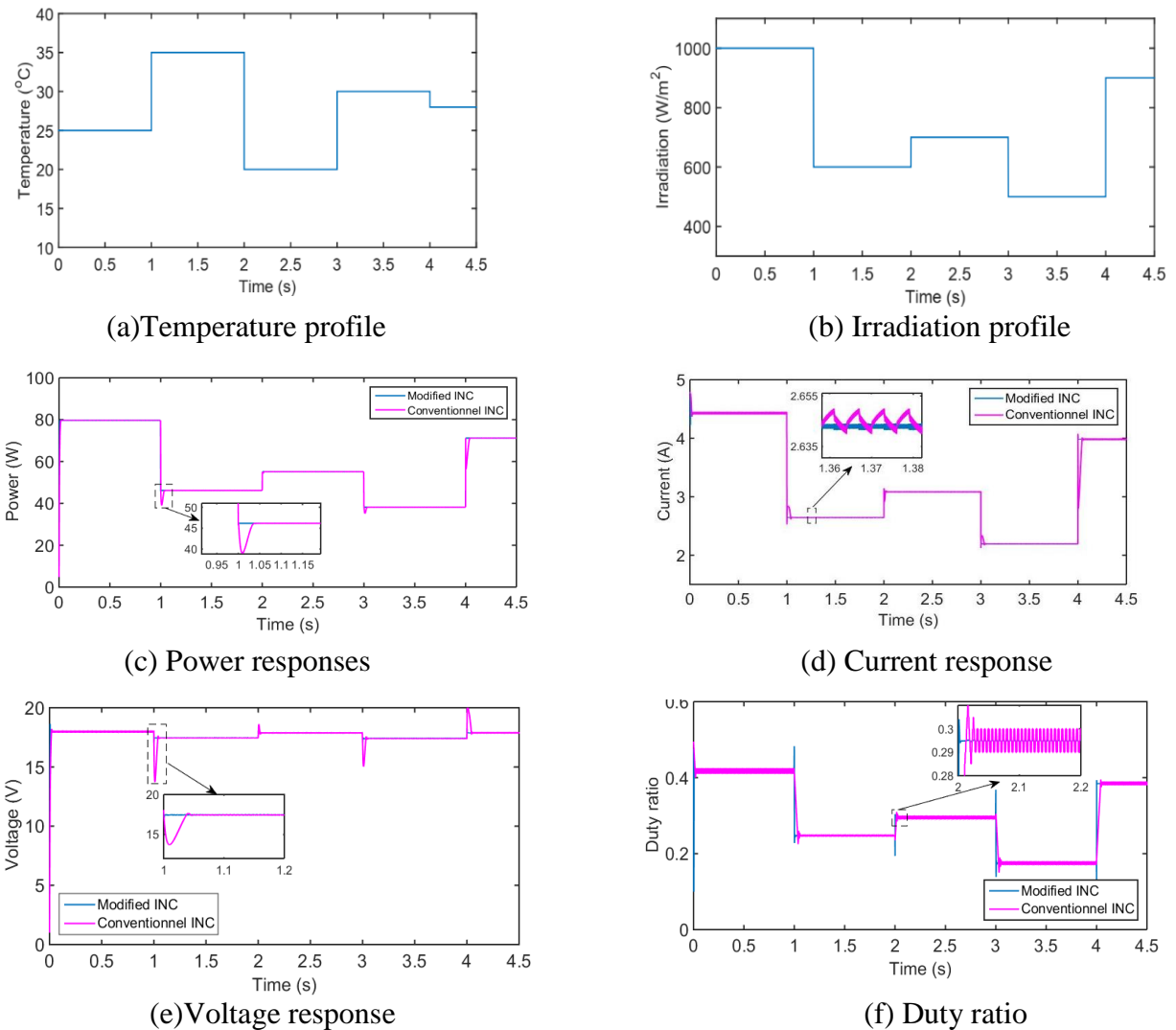
Fig. 8. Simulation results for PV system under varying environmental conditions
