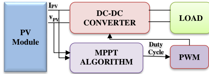
Fig.1 PV system control structure.
