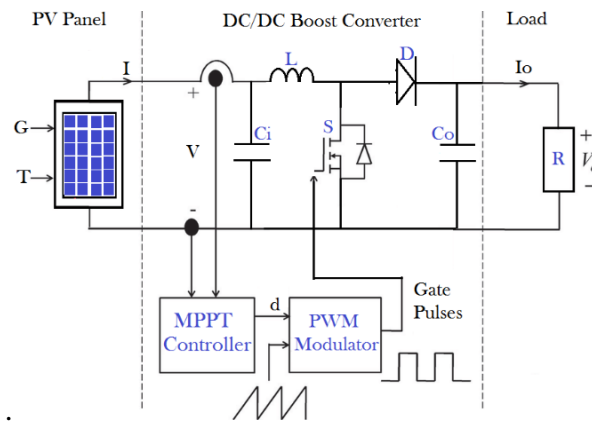
Fig. 4. DC-DC boost converter circuit.
