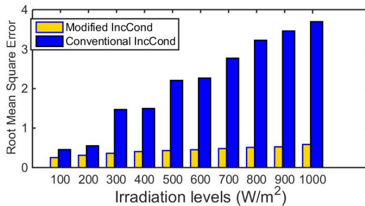
Fig. 9. RMS errors at different irradiancies and constant temperature
