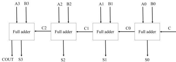
Figure 5. The proposed schematic for 4-bit RCA
