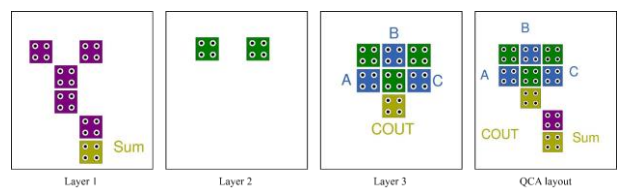
Figure 4. QCA-based full adder layouts and layers
