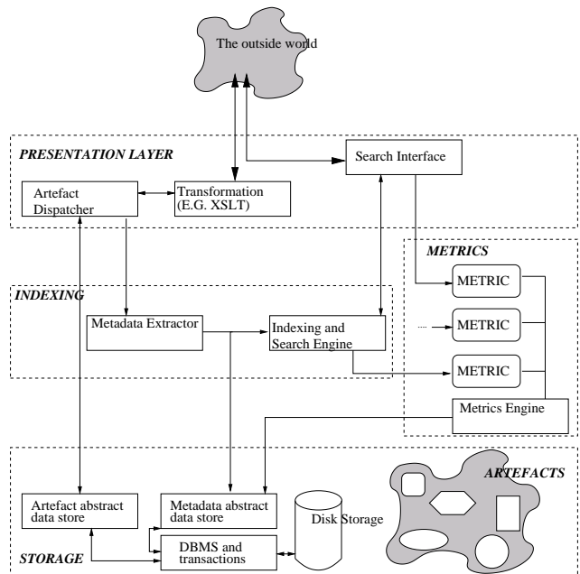
Figure 1. OSCAR Architecture
