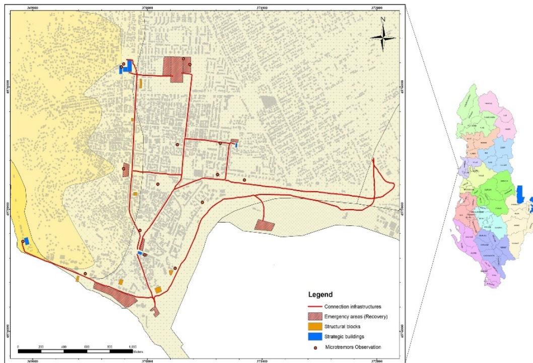
Figure 1. Shows the integrated approach of the SMS and the LCE for the center of the city of Durrës.
