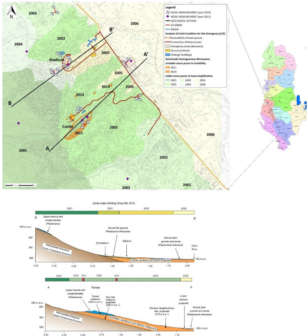
Figure 2. The conjugate approach of the SMS and the LCE of the city of Gjirokastra, allows the systematic association of strictly geological information with the strategic elements functional to emergency management. Basemap is the Seismically Homogeneous Microzones Map modified from Cavinato et al., 2014. Codes 2001:2006 and 3011-3014 are defined according to the Working Group SM, 2015 guidelines [9].
