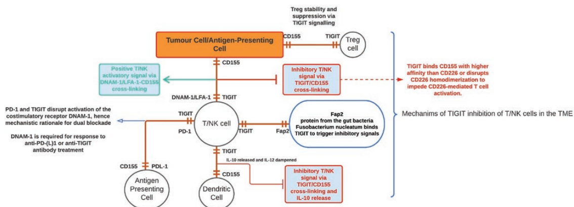
Figure 1. Interplay in the TIGIT/CD155/DNAM-1 axis.
