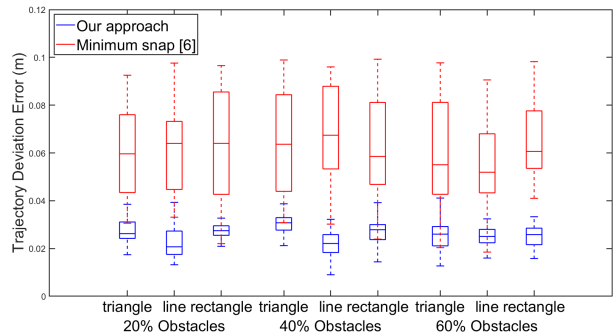
Fig. 8. The average trajectory deviation error of our approach against minimum snap [6].
