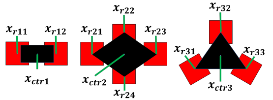
Fig. 3. Linear, rectangular, and triangular formations consisting of several robots (in red) and an object (in black). Each robot i is placed with its state \mathbf{x}_{rj} relative to the j th formation's centroid state \mathbf{x}_{ctrj} .
