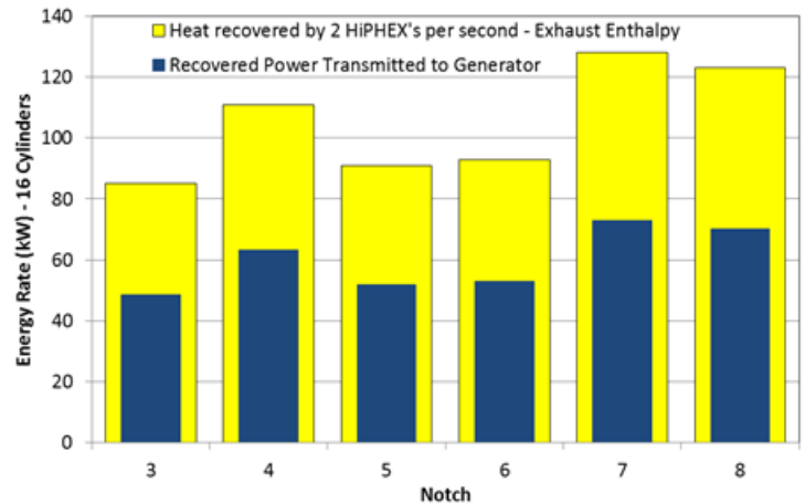
Electrical Energy Recovered with HiPHEX
