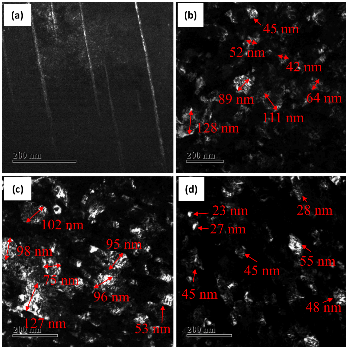
Fig. 11. Representative TEM DF micrographs showing the extent of microstructural refinement: (a) 1/2 turn- center, (b) 1/2 turn- edge, (c) 5 turns- center, (d) 5 turns- edge.
