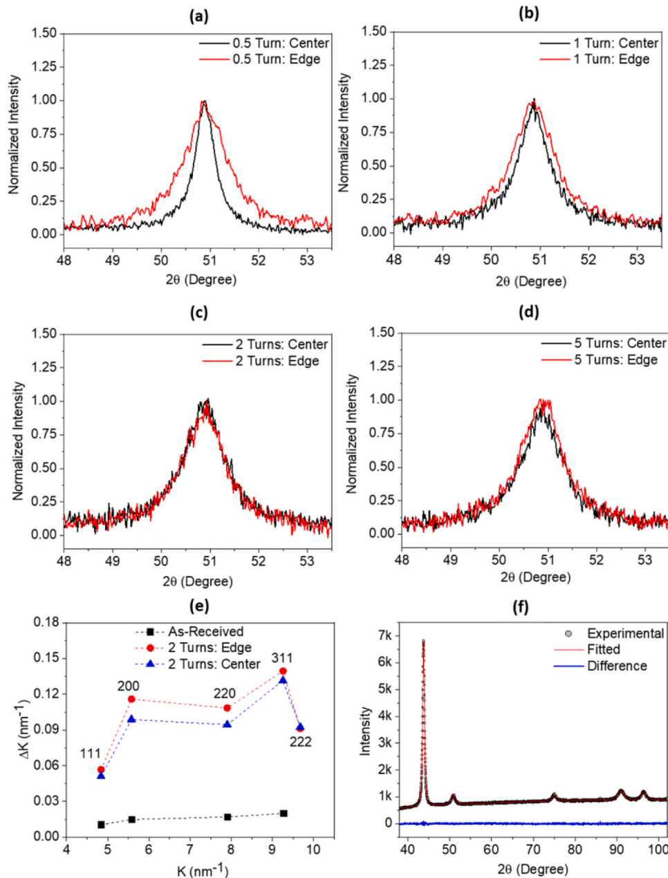
Fig. 5. Illustration of XRD peak broadening at center and edge for (200) peak: (a) \frac{1}{2} turn, (b) 1 turn (c) 2 turns, (d) 5 turns, (e) WH plot for the samples in as-received condition and at center and edge locations after 2 turns of HPT, (f) experimentally determined and fitted XRD pattern using CMWP method for 5 turns at edge location.
