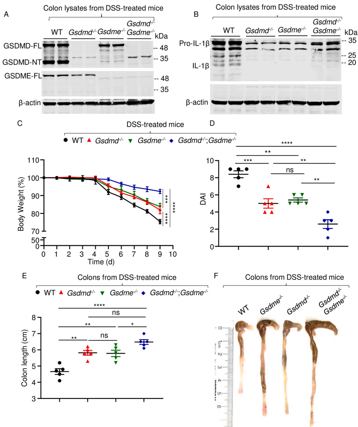
Fig. 1. Loss of GSDMD or GSDME attenuated DSS-induced colitis. Mice were administrated with 2.5% DSS in drink water for 9 days. (A and B) Colon lysates were analyzed by immunoblotting. (C) Mouse body weight, recorded daily. (D) DAI. (E) Colon length. (F) Representative images of the colons. Data are mean ± SEM. N = 5 mice/group. * p < 0.05; ** p < 0.005; *** p < 0.0005; **** p < 0.0001. One-Way ANOVA or Two-Way ANOVA. DAI, disease activity index; FL, full-length; ns, non-significant; WT, wild-type.
