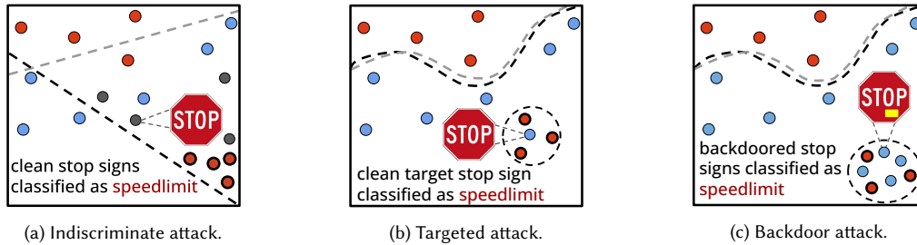
Fig. 4. Conceptual representation of the impact of indiscriminate, targeted, and backdoor poisoning on the learned decision function. We depict the feature representations of the speed limit sign (red dots) and stop signs (blue dots). The poisoning samples (solid black border) change the original decision boundary (dashed grey) to a poisoned variant (dashed black).
