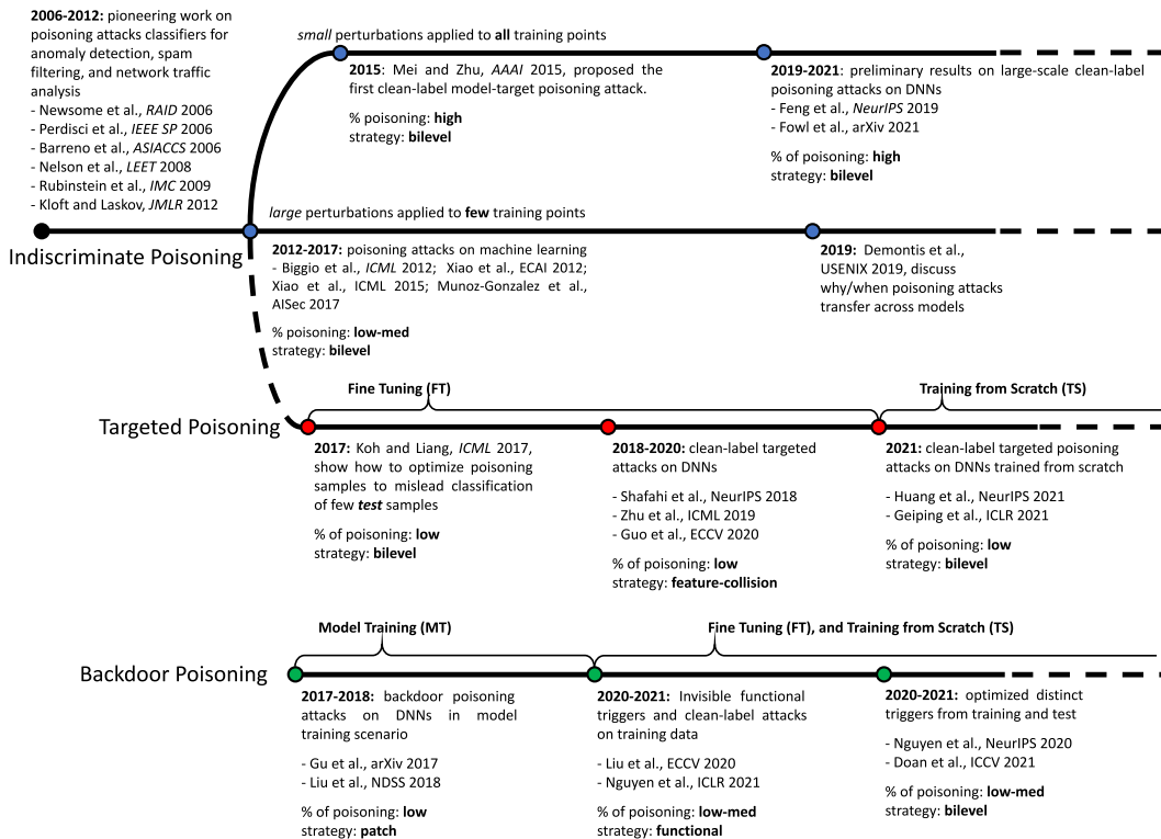
Fig. 5. Timeline for indiscriminate (blue), targeted (red) and backdoor (green) data poisoning attacks on machine learning. Related work is highlighted with markers of the same color and connected with dashed lines to highlight independent (but related) findings.
