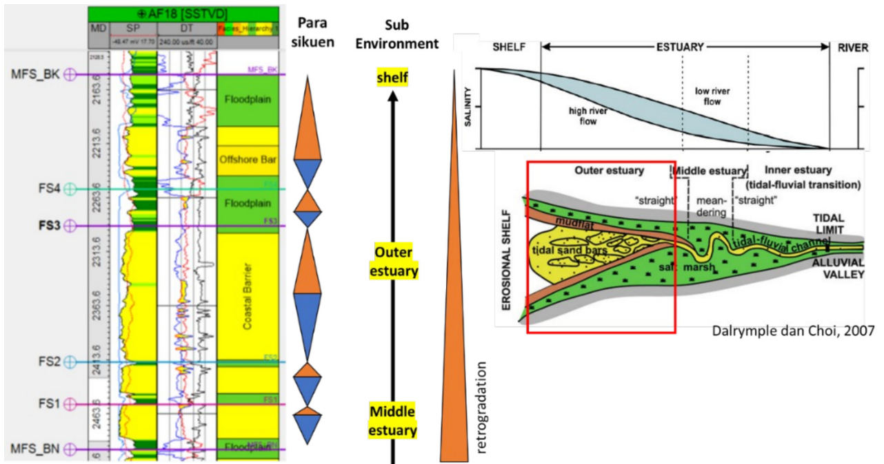
FIGURE 6. Four stratigraphic markers (flooding surface) were identified by shale break barrier and interpreted estuarine environment with tide influences at Bekasap Formation (Dairymple and Choi, 2007). The dynamic sedimentation from the lower to the top gave a retrogradation pattern and illustrated the area getting to the shelf environment. All lithology shale (green color) interpretations can be considered floodplain, mudflat, or marine shale (non-reservoir zone), and the zone below MFS_BK is interpreted as marine shale.
