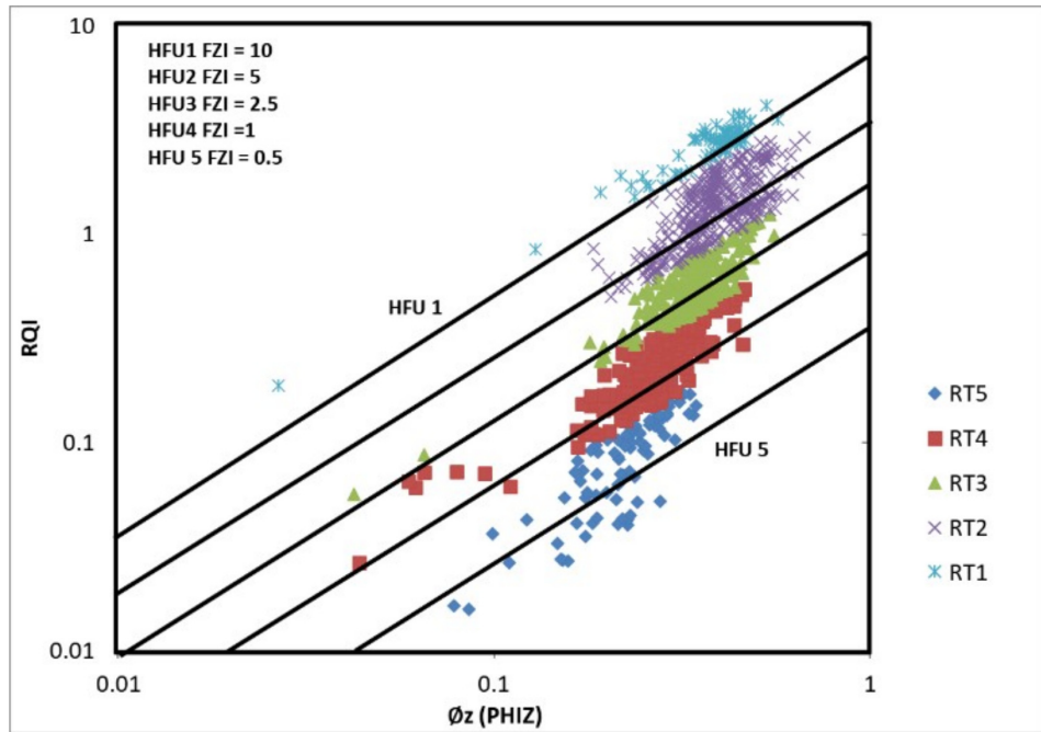
FIGURE 13. Hydraulic Flow Units by plotting porosity normalized (PHIZ) and reservoir rock quality (RQI).
