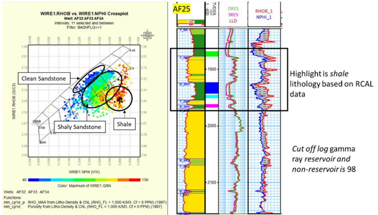
FIGURE 5. Three lithotypes (clean sandstone, shaly sandstone, and shale) types were identified in Bekasap Formation. Density and neutron cross-plot was used to cut off the GR log and got 30–98 gAPI as the reservoir zone (sand), and the upper 98 gAPI was non-reservoir (shale).
