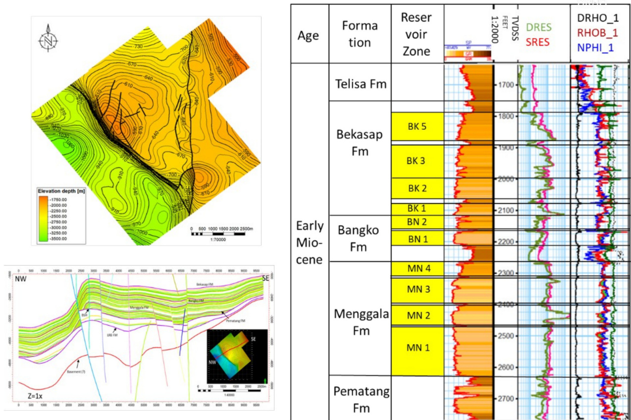
FIGURE 2. The structural map at Top Bekasap Formation and a cross-section through AF Field showed some fault configuring the Area. Stratigraphic succession and reservoir identification at Bekasap (BK), Bangko (BN), and Menggala (MN) Formation (LKFT UGM, 2021).
