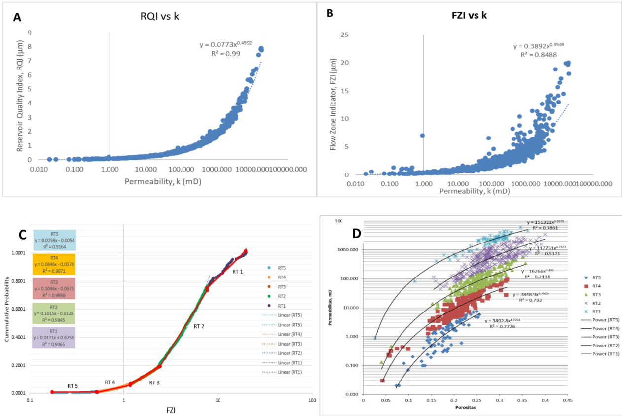
FIGURE 12. A. Cross plot between RQI versus permeability ( k ); B. Cross plot between FZI versus permeability ( k ); C. Rock type division based on FZI ; D. Cross plot between porosity ( PHIE ) versus permeability ( k ). All figures explain the reservoir quality index ( RQI ) and Flow Zone Indicator ( FZI ) between porosity and permeability.
