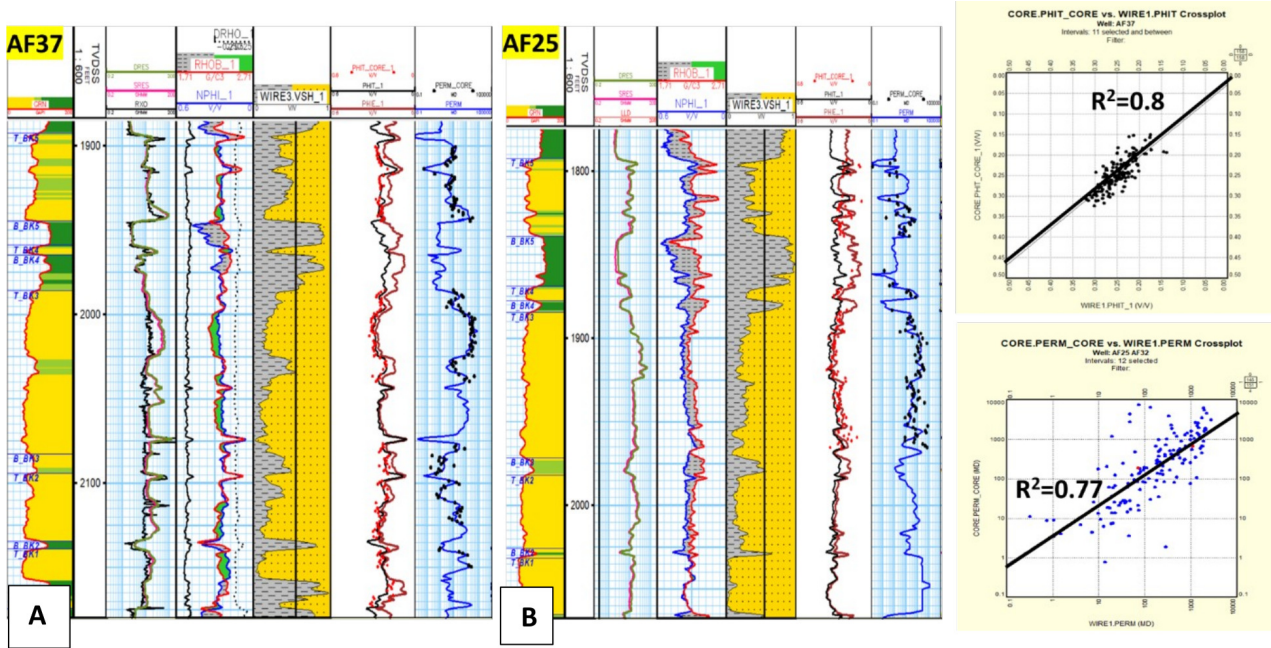
FIGURE 9. (a) Porosity calculation at AF 37 wells and got the close correlation as 0.8 and (b) Permeability calculation using Wyllie formula and got correlation factor as 0.77 with core data (RCAL).
