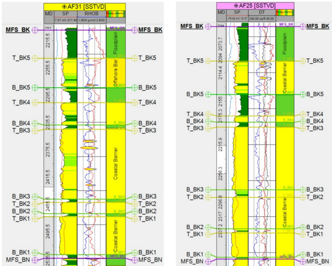
FIGURE 7. Five reservoir zonation (BK1, BK2, BK3, BK4, and BK5) were identified by composite log responses where regional markers bounded upper and lower formations.
