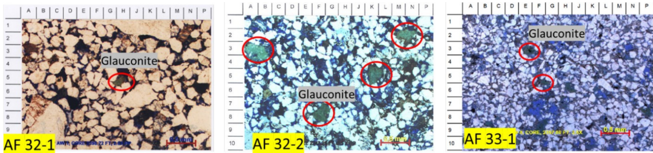
FIGURE 4. In thin section analysis at AF Field in Bekasap Sand Reservoir, the grain from left to right was decreased (fine-grained - very fine-grained) with moderately to poorly sorted. The detrital grains are dominated by quartz and rock fragments. The presence of glauconite, pyrite, and clay minerals is observed as accessory minerals (Lemigas, 2013).
