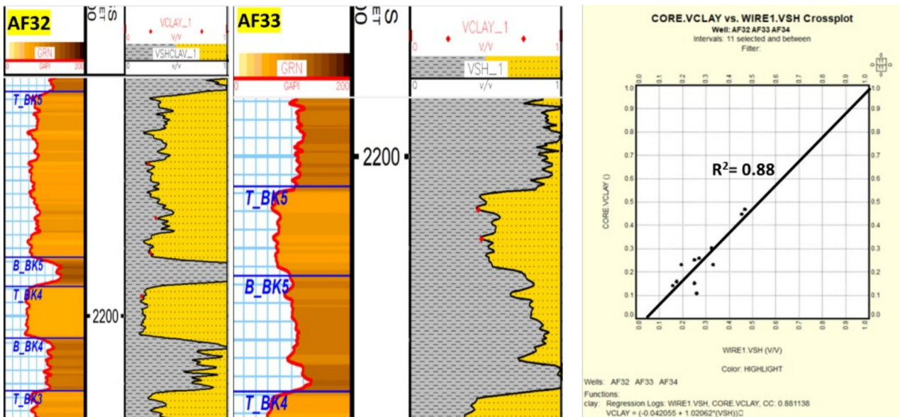
FIGURE 8. Shale volume calculation at AF32 and AF33 with validated data from core data (XRD analysis) gave a good correlation of 0.88.
