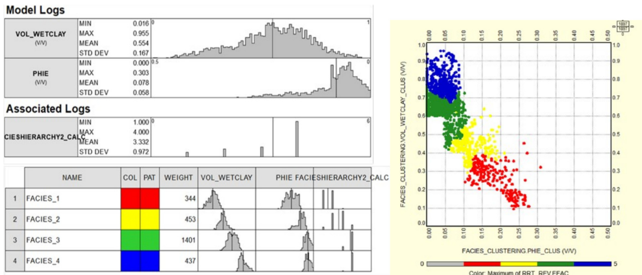
FIGURE 14. Clustering analysis at AF Fields using MRGC method and resulting four facies (rock type).
