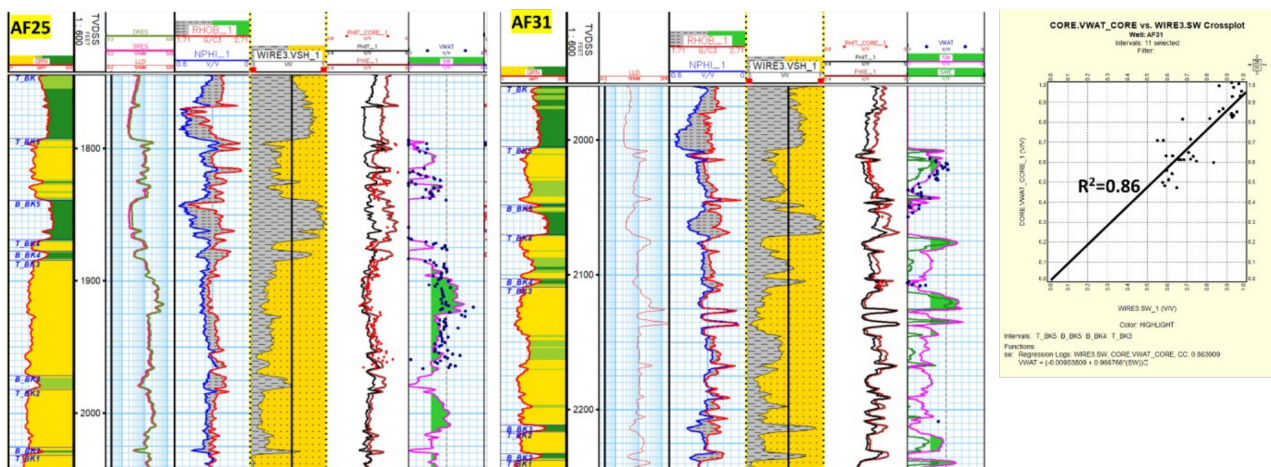
FIGURE 10. Water saturation calculation using the Simandoux formula is suitable for shaly sand reservoirs such as BK 5 and BK4. The correlation between log analysis and core measurement is 0.86.
