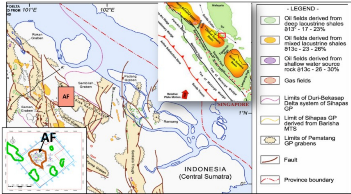
FIGURE 1. The Sitemap of Central Sumatra Basin shows the AF Field Association’s location with another field in Riau Province, Indonesia. The geological map recognized features and hydrocarbon potential in the Central Sumatra Basin from Heidrick and Aulia (1993) and Pertamina BPPKA (1996).
