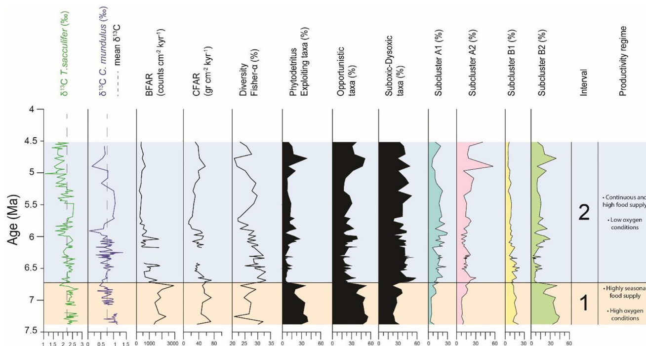
Figure 6. Benthic and planktonic stable carbon isotope records, BFAR, CFAR, diversity (Fisher- \alpha index), relative abundance of phytodetritus exploiting taxa, opportunistic taxa, suboxic-dysoxic taxa, and subclusters plotted against age (Ma). Highlighted Interval 1 (orange), Interval 2 (blue) indicate the productivity regimes.
