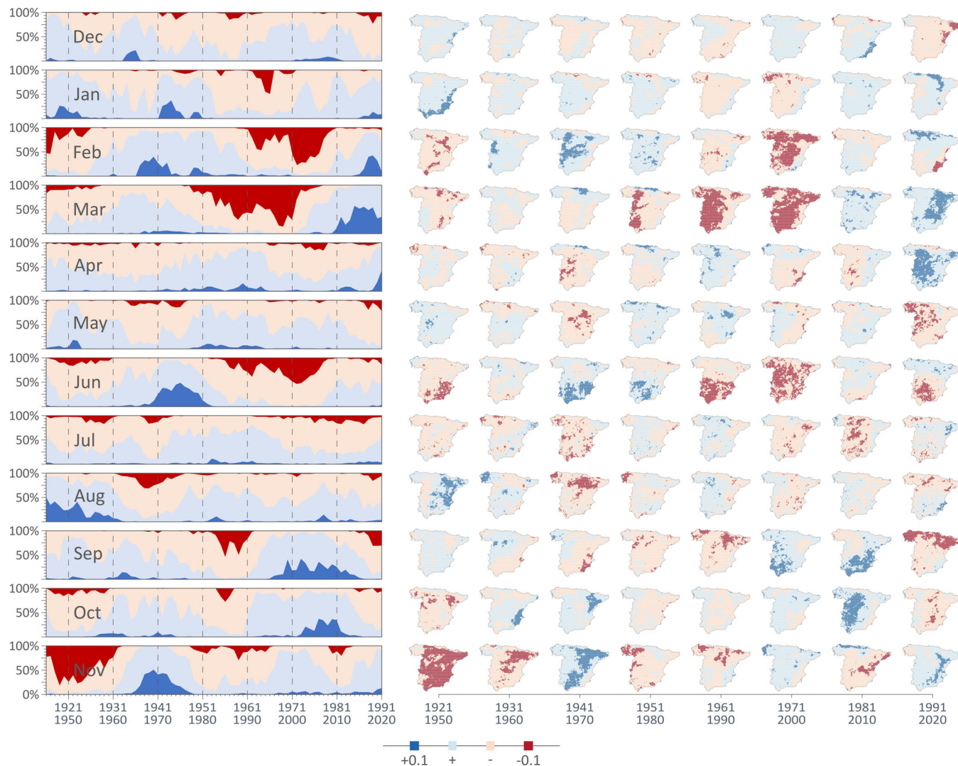
FIGURE 6 Percentage of grid cells according to their trend sign and significance under 30-year temporal windows from 1916–1945 to 1991–2020, in 1-year increments. Legend as in Figure 2
