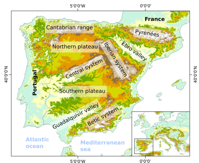
FIGURE 1 Study area and the main spatial distribution of mountain chains
