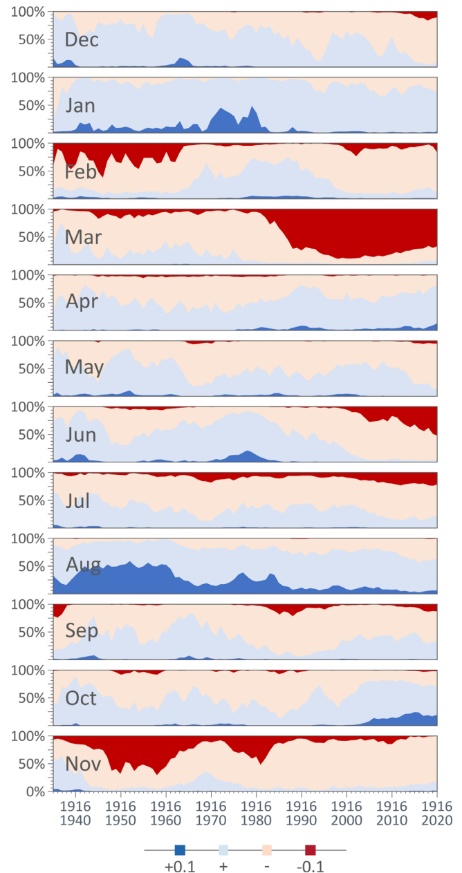
FIGURE 3 Percentage of grid cells according to their trend sign and significance under increasing temporal windows from 1916–1935 to 1916–2020, in 1-year increments. Legend as in Figure 2
