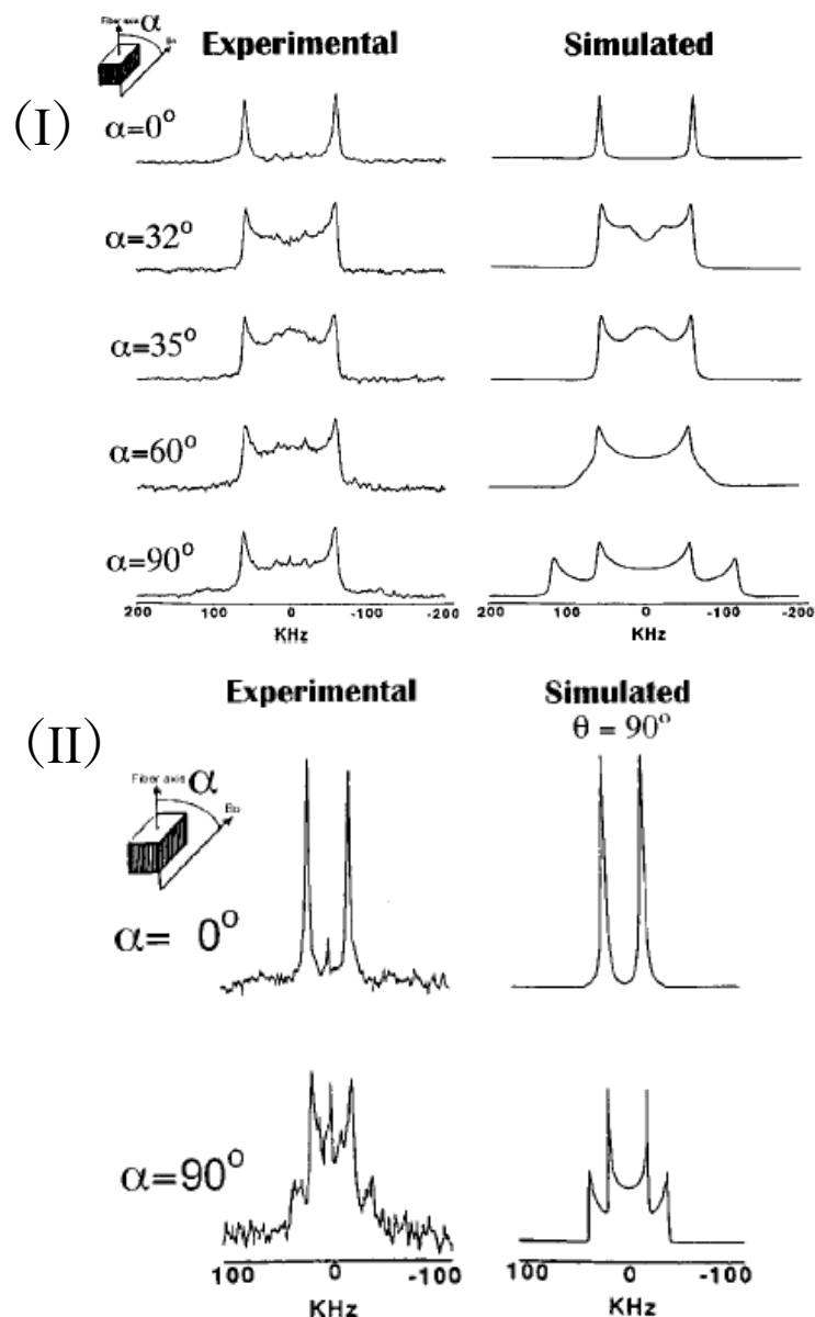
Figure 13. Experimental and simulated ^2\text{H} solid-state NMR spectra of uniaxially aligned (I) [2,2\text{-}^2\text{H}_2]\text{Gly-} and (II) [3,3,3\text{-}^2\text{H}_3]\text{Ala-SF} fibers. The angle \alpha between the fiber axis and magnetic field was set to be (I) 0^\circ , 32^\circ , 35^\circ , 60^\circ and 90^\circ , and (II) 0^\circ and 90^\circ . When the angle between the \text{C}\alpha\text{-}^2\text{H}_2 bond of Gly and fiber axis was assumed to be 90^\circ , the experimental spectra could be well simulated as shown in (I). Similarly, a good agreement was also obtained when the angle between the \text{C}\alpha\text{-C}\beta^2\text{H}_3 bond of Ala and the fiber axis was assumed to be 90^\circ for (II). Adapted with permission from Asakura et al., ^2\text{H} -Labeling of Silk Fibroin Fibers and Their Structural Characterization by Solid-State ^2\text{H} NMR. Macromolecules 1997, 30, 2429-2435. Copyright 1997 American Chemical Society.
