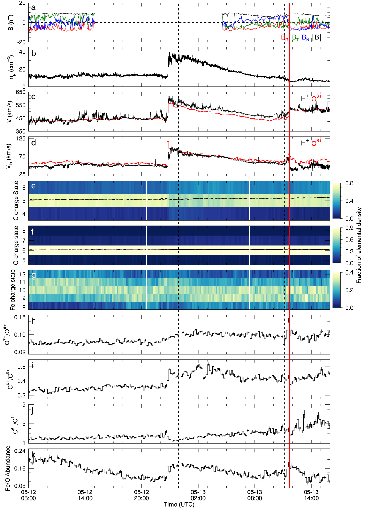
Fig. 3. In situ measurements of an event in the solar wind on 12 to 13 May 2022. (a) MAG magnetic field RTN components and magnitude, (b) PAS n_p , (c-d) PAS v_p and v_{p,th} and HIS v_{O^{6+}} , and v_{O^{6+,th}} , (e-g) elemental charge state distributions of C, O, Fe, (h-j) ion charge state ratios, and (k) Fe/O element abundance ratio. The first solid vertical red line marks the shock arrival time as observed by HIS. The ICME region is bounded vertical dashed black lines. A reverse shock is marked by the second solid vertical red line.
