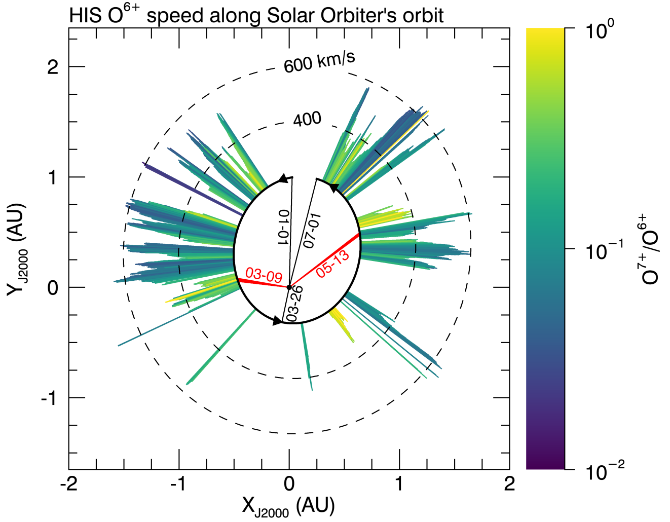
Fig. 5. HIS observations of O^{6+} bulk speed (vector length) and O^{7+}/O^{6+} ratio (vector color) over Solar Orbiter's first science orbit from January – June 2022. Perihelion and interval start+stop dates are labeled in black and the event dates from Figures 3 and 4 are labeled in red.
