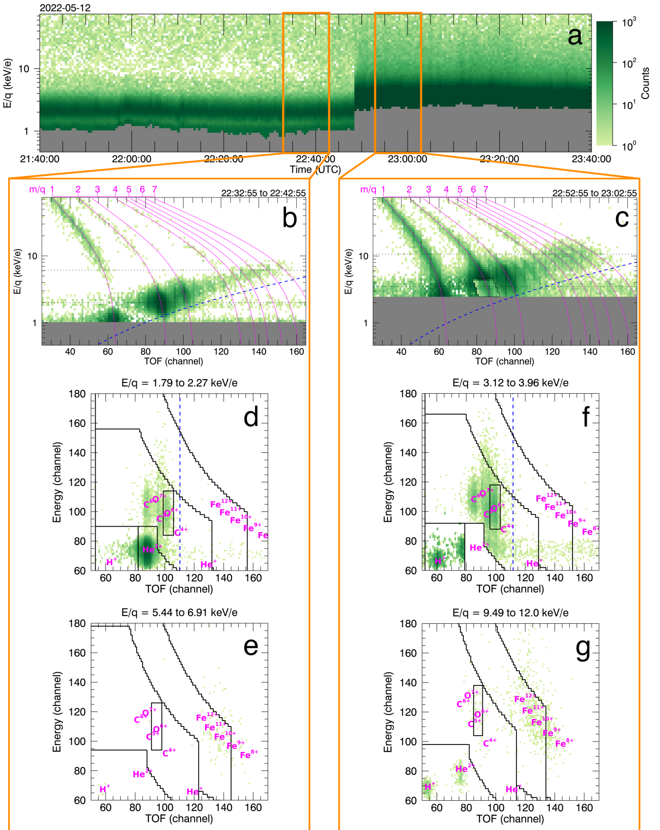
Fig. 2. HIS measurements about an interplanetary shock encountered by Solar Orbiter on 12 May 2022. a: HIS E/q spectra at native 30-second resolution over a 2 hour interval. b-c: E/q-TOF distributions accumulated over 10-min before and after the shock, corresponding respectively to the orange-outlined intervals in a. Panels d-g: E-TOF distributions at the peak E/q step for He^{2+} and other M/q = 2 ions (d and f) and for Fe^{9+} (e and g). The colorbar is consistent throughout all panels. Dark gray indicates E/q steps affected by the instrument's proton avoidance (a-c), magenta corresponds to m/q (b-c) and ion species (d-g), dashed blue lines are the velocity filter applied to the data (b-g), and thick black lines mark boundaries between priority ranges as listed in Table 1 (c-g). Suprathermal trails for (left to right in TOF) H^{1+} , He^{2+} , and He^{1+} can be observed in (b, c).
