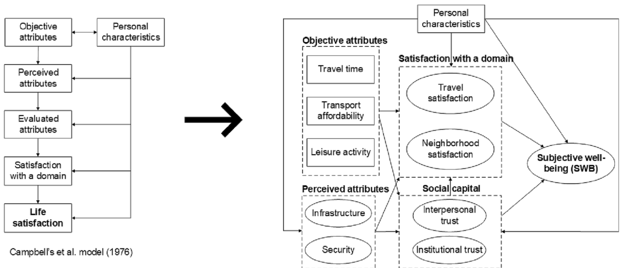
Fig. 1. Conceptual model.
