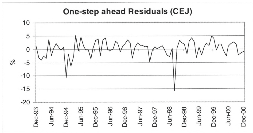
Figure 3.6. One-step-ahead Residuals calculated for the CEJ model.
