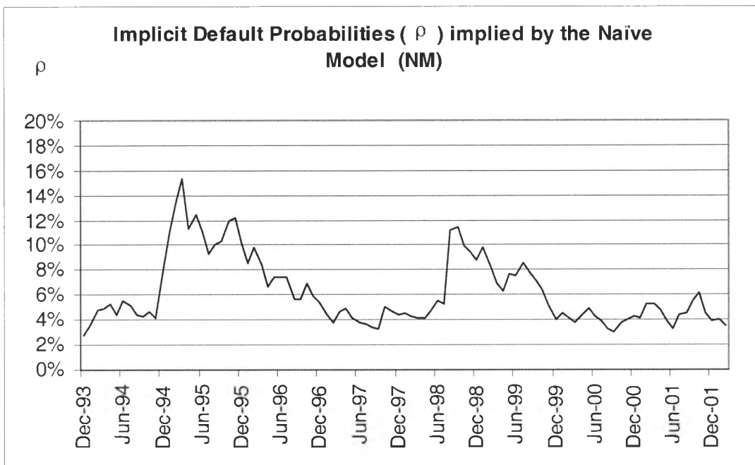
Figure 3.2. Implicit Probabilities of Default \rho_t
