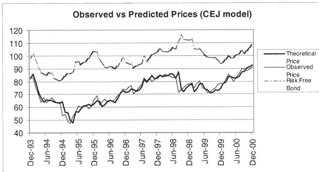
Figure 3.5. Actual against Fitted Prices
