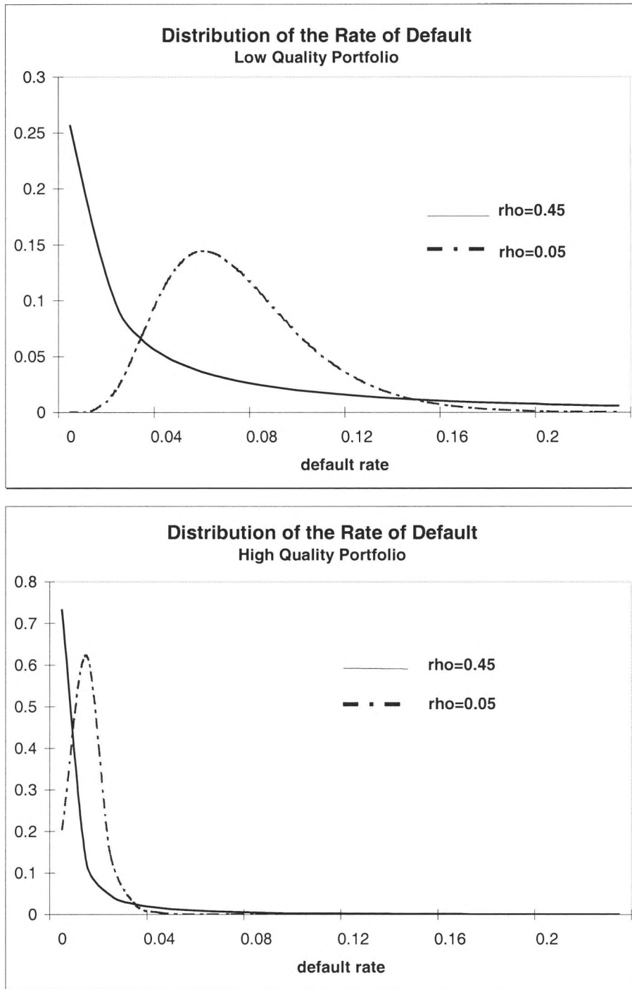
Figure 5.2. Default Rate Distributions for CreditMetrics. Low-Quality (LQ) and High-Quality(HQ) Portfolios
