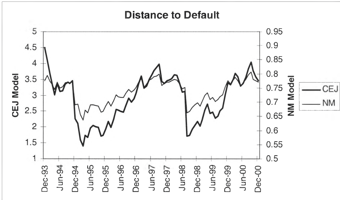
Figure 3.3. Distance-to-Default implied by the Models The variables correspond to the updated estimates of the Kalman Filter
