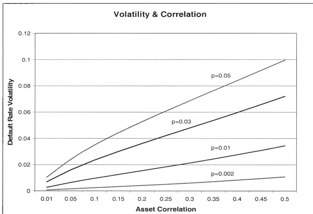
Figure 5.1. Consistent Parameters for CreditMetrics and CreditRisk+
