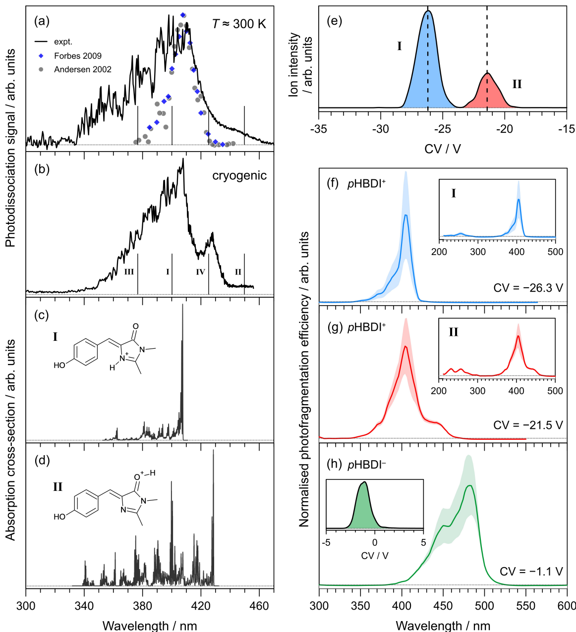
Fig. 2 Action spectroscopy of p\text{HBDI}^+ : (a) photodissociation spectrum at T \approx 300\text{ K} [grey dots taken from Ref. 24 and blue diamonds from Ref. 26], (b) photodissociation spectrum at cryogenic temperature. Vertical bars indicate the calculated vertical excitation wavelengths for protomers I–IV, determined at the DLPNO-STEOM-CCSD(T)/aug-cc-pVDZ level of theory. Franck-Condon simulation of the S_1 \leftarrow S_0 absorption profiles (at T = 20\text{ K} ) for: (c) protomer I (lowest energy protomer) assigned as the imine protomer I in Fig. 1, and (d) protomer II (second lowest energy protomer) assigned as the carbonyl protomer II in Fig. 1. Protomer-specific photodissociation action spectroscopy: (e) ionogram recorded using DMS heated to 150^\circ\text{C} with 1.5 mol% acetonitrile entrained in \text{N}_2 at \text{SV} = 3500\text{ V} showing two isomer populations, assigned to protomers I and II, (f) photodissociation spectrum for protomer I, (g) photodissociation spectrum for protomer II. Panel (h) shows the photodissociation spectrum recorded for (deprotonated) p\text{HBDI}^- and ionogram (inset), consistent with a single deprotonated [SV = 3000\text{ V} , pure \text{N}_2 carrier gas], and with earlier spectra. 22,54 Dotted horizontal baselines indicate the zero signal level.
