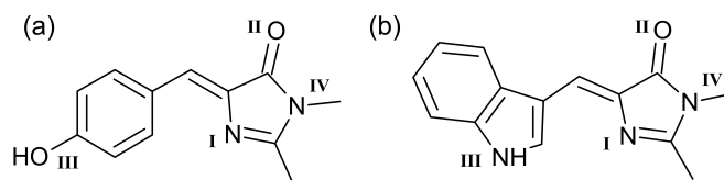
Fig. 1 Structure of (a) p HBDI and (b) Cyan. The protonated cations are denoted p HBDI + and Cyan + , with the four possible protonation sites identified. In both cases, protonation site I (imine) corresponds to the lowest energy protomer. Each protomer may have E and Z geometric configurations about the double bond on the methine bridge. In all cases, the Z isomer is lower in energy. The E isomer, if present, is expected in only trace quantities.
