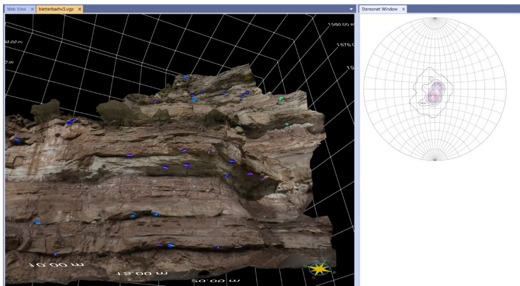
Figure 2. Strata beds and related contour-plot showing a mainly horizontal attitude.
