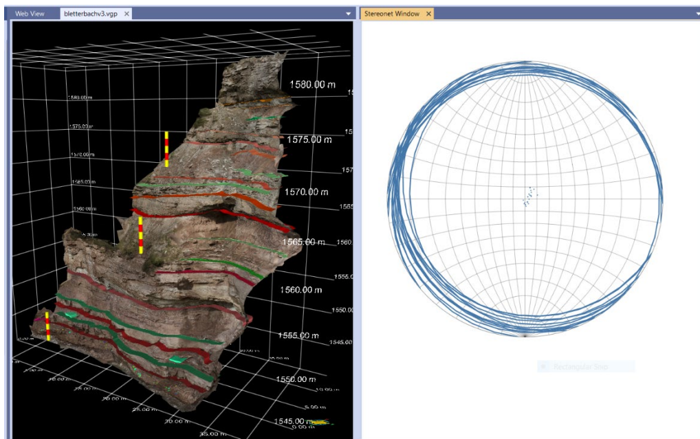
Figure 4. Digital outcrop model (DOM) Interpretation as in figure 1 and stereo-plot (great circles) of the main facies boundaries (almost horizontal)
