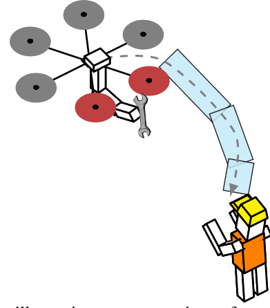
Fig. 3: An illustrative representation of an MRV approaching a human operator. In blue are depicted the areas (\underline{p}_{\text{pr}}^{(j)}, \bar{p}_{\text{pr}}^{(j)}) where the drone can approach the operator, while in gray is a sample output from the STL optimizer.
