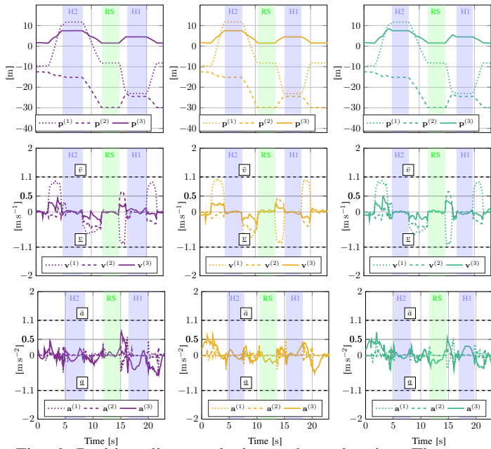
Fig. 6: Position, linear velocity, and acceleration. The trajectories are shown for the different operators' preferred approach directions, including left and right (left), front (middle), and top to bottom (right). The time frames for handover and refilling are indicated using blue and green colors, respectively.
