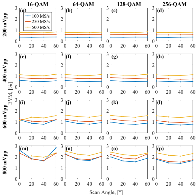
Fig. 6. TX EVM vs. scan angle measured over-the-air at a 3 m TX-RX separation for various modulated transmissions (increasing order from left to right) and various input signal voltages of the AWG (increasing order from the top down) at three transmission rates, i.e., 100, 250, 500 MS/s.
