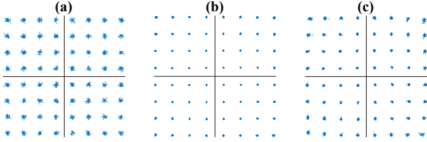
Fig. 4. Measured constellation errors for a 64-QAM modulated transmission at 500 MS/s (equivalent to 3 Gbps transmission rate) (a) EVM=3.1 % and EIRP=18 dBm, (b) EVM=1.2 % and EIRP=55 dBm, and (c) EVM=2.6 % and EIRP=60.5 dBm (at 5 dB back-off from saturation). See Fig. 3 for OTA measurement.
