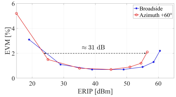
Fig. 5. TX EVM vs. EIRP measured over-the-air at a 3 m TX-RX separation for a 64-QAM modulated transmission at 250 MS/s (equivalent to 1.5 Gbps transmission rate) at the indoor measurement setup shown in Fig. 3.
