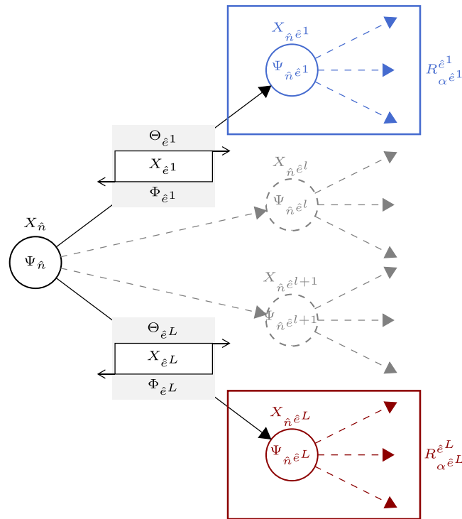
Figure 3. The recursive representation of a regularization graph according to lemma 3.2.
