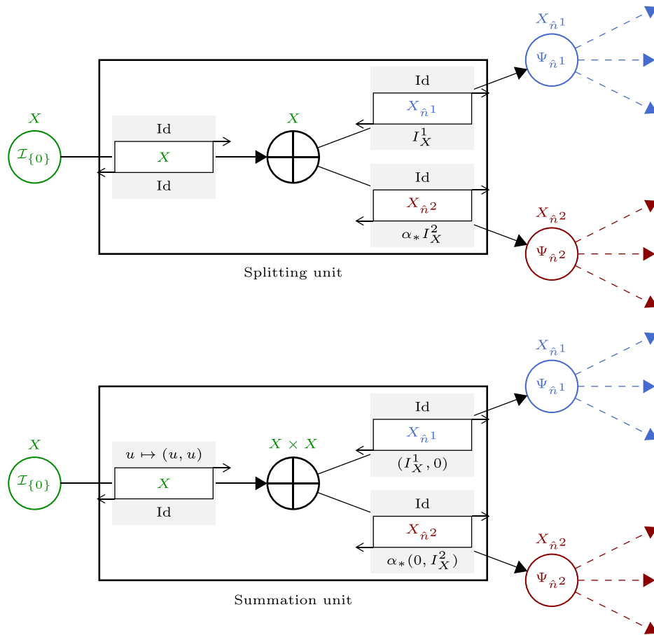
Figure 4. Combining regularization graphs via infimal convolution (top) and summation (bottom).
