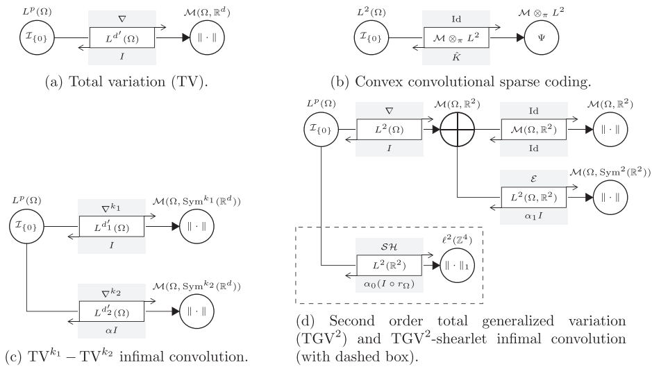
Figure 2. Examples of regularization graphs reproducing existing regularization functionals.
