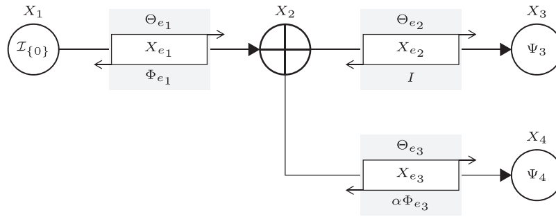
Figure 1. Example of a regularization graph with nodes V = \{1, 2, 3, 4\} , edges E = \{(1, 2), (2, 3), (2, 4)\} = \{e_1, e_2, e_3\} and weights (\alpha_{(1,2)}, \alpha_{(2,3)}, \alpha_{(2,4)}) = (1, 1, \alpha) . See remark 2.5 for a detailed interpretation.
