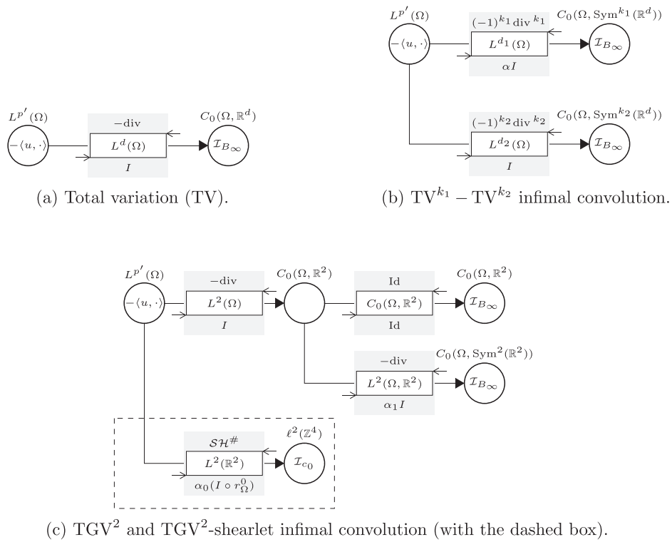
Figure 5. Examples of predual regularization graphs.
