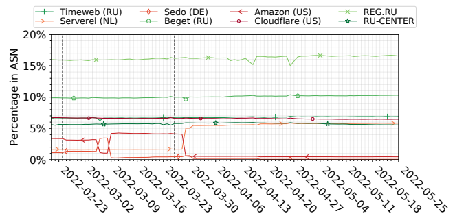
Figure 4: Hosting networks of .ru and .pf domain names (Top ASNs). The share of Russian domain names that each network hosts is shown. The vertical dashed lines delineate the pre-conflict , pre-sanctions and post-sanctions periods.
