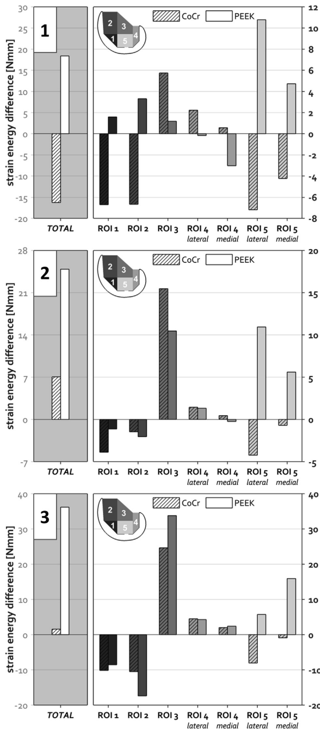
Fig. 5. Postoperative volumetric strain energy density differences in all specimens, separated for five periprosthetic regions of interest. The SED values at each integration point in a specific ROI were multiplied by their volume and summed to yield the total strain energy per ROI.
