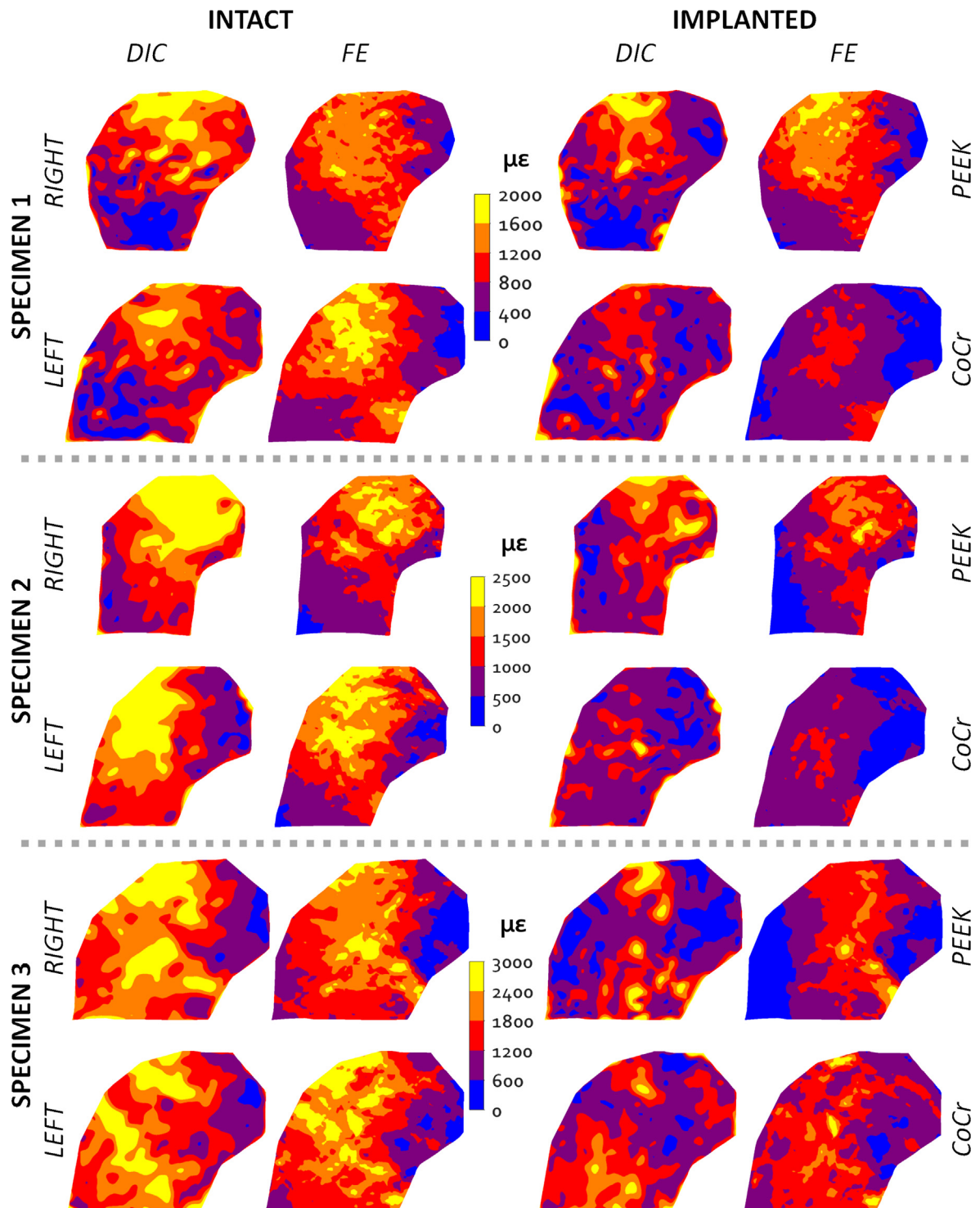
Fig. 3. Von Mises strain maps of all specimens for both pre- and postoperative DIC and FE measurements.
