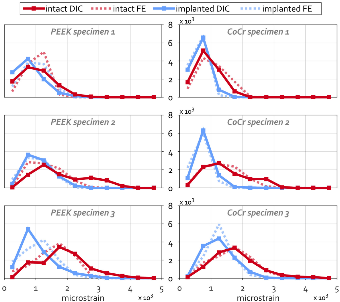
Fig. 4. Von Mises surface strain distributions for both pre- and postoperative DIC and FE measurements. The strains are determined at the surface sampling points and accumulated in 500 microstrain intervals.
