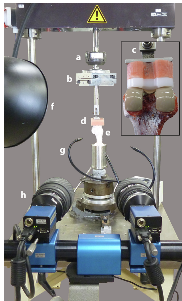
Fig. 1. Experimental setup with a) the load cell, b) planar x/y bearing, c) varus/valgus hinge (in inset), d) custom load applicator, e) painted specimen, f) ambient light source, g) focal light source, h) dual camera setup.
