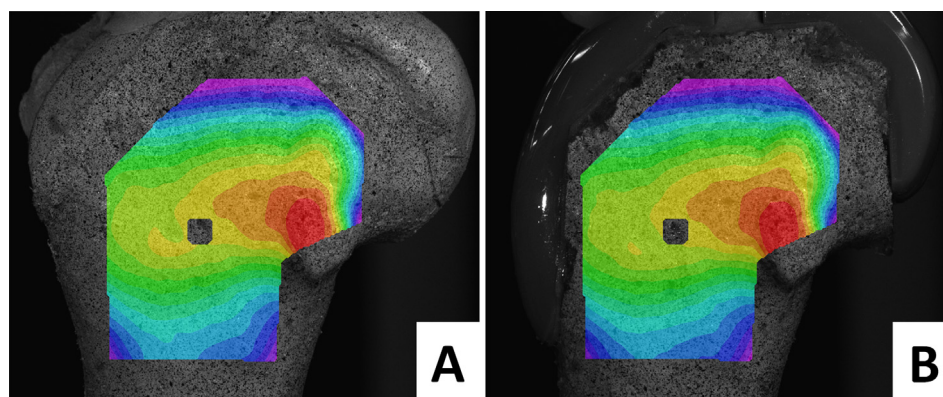
Fig. 2. DIC region of interest surface topology on (A) the intact femur and (B) the implanted femur. The region is chosen such that the speckle patterns are visible in both trials.
