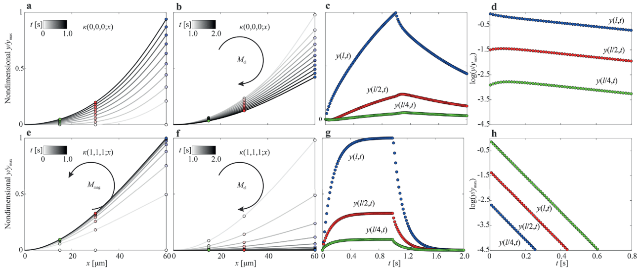
Figure 4. Simulation results of two flagella of bending stiffness \langle \kappa(0, 0, 0) \rangle and \langle \kappa(1, 1, 1) \rangle . Parameters: \eta = 1 \text{ mPa}\cdot\text{s} , l = 60 \mu\text{m} , d_f = 1 \mu\text{m} , l_m = 13 \mu\text{m} , l_p = 40 \mu\text{m} , and l_d = 7 \mu\text{m} . Darker curves indicate later times. a–d) The passive flagellum is driven by distal contact force. The force is removed and the elastic moment restores its original shape. Position of the filament at l , l/2 , and l/4 are calculated versus time and the decay time T is calculated from the slope of \log(y) . The average decay rate is 1/T(0, 0, 0) = 0.7 \text{ s}^{-1} . e, h) The passive flagellum is driven by magnetic field and nanoparticle coating. Energy is fed in by a magnetic torque through a distribution B(1, 1, 1; x) . The flagellum returns to its original shape when the applied field is removed. The decay rate is 1/T(1, 1, 1) = 7.2 \text{ s}^{-1} .
