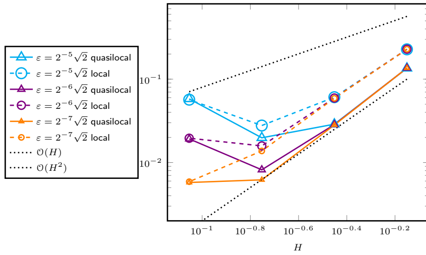
Figure 4: Relative errors \|\mathbb{E}[\mathbf{u}_h] - u_H\|_{L^2(D)} (quasilocal) and \|\mathbb{E}[\mathbf{u}_h] - \tilde{u}_H\|_{L^2(D)} (local) in dependence of the coarse mesh size H .
