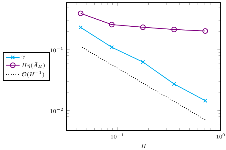
Figure 3: Model error estimators H for \varepsilon = 2^{-7}\sqrt{2} .
