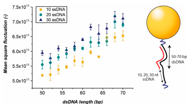
Figure 4. Mean square fluctuation of the maximum detector signal for different tether properties where n = 3 individual simulations for each data point. Error bars represent the mean \pm sd, where n = 3 (three independent simulations).
