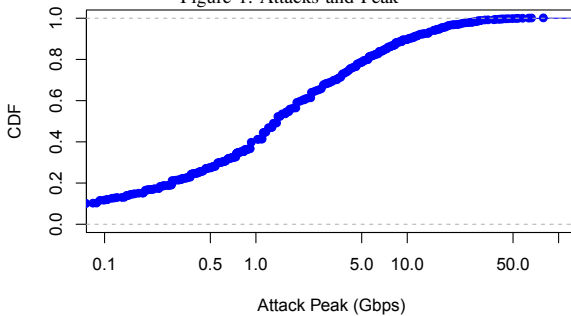
Figure 2. CDF of Attack Rates (peak)
