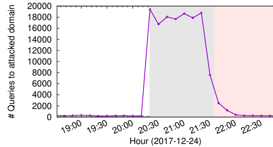
Figure 11. Timeseries of queries to .nl for single targeted domain of share hosting from Figure 10.
