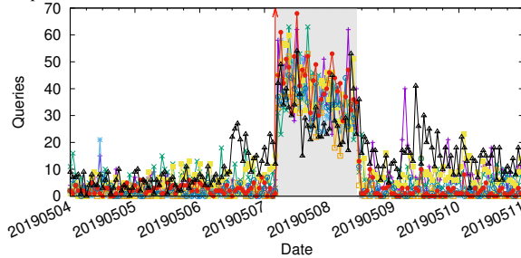
Figure 13. Timeseries of queries to 8 targeted .nl domains
