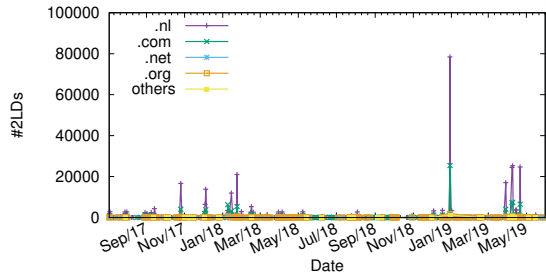
Figure 6. Time series of affected second-level domains per TLD
