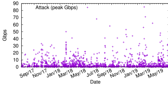
Figure 1. Attacks and Peak
