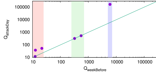
Figure 10. [IP-Date] shared hosting 6 .nl domains and number of queries with one targeted domain
