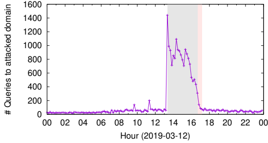
Figure 9. Timeseries of incoming queries to .nl for dedicated hosting domain. Pink area show area which scrubbing service was active; gray area shows when attacked started being noticed on DNS
