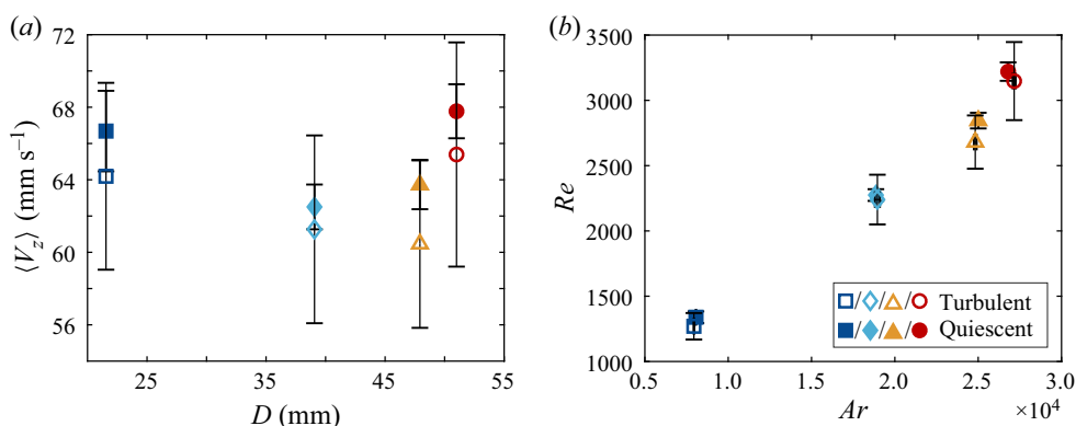
Figure 13. (a) Mean descent velocities \langle V_z \rangle of the various particles in turbulence and quiescent fluid. (b) Dimensionless version of the descent velocity plot, Re(Ar) .
